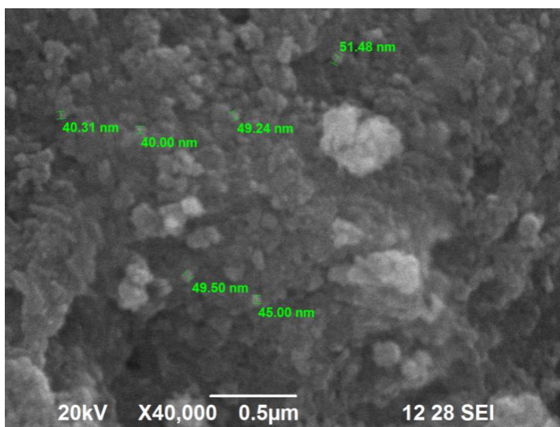
Figure 6. Scanning electron microscope spectra of iron oxide magnetic nanoparticles
