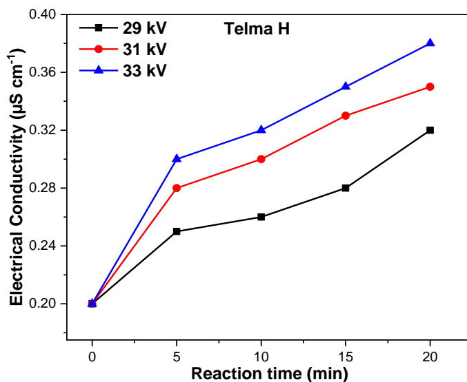
Fig 7. APPJ treated T-H aqueous solution Electrical conductivity graph
