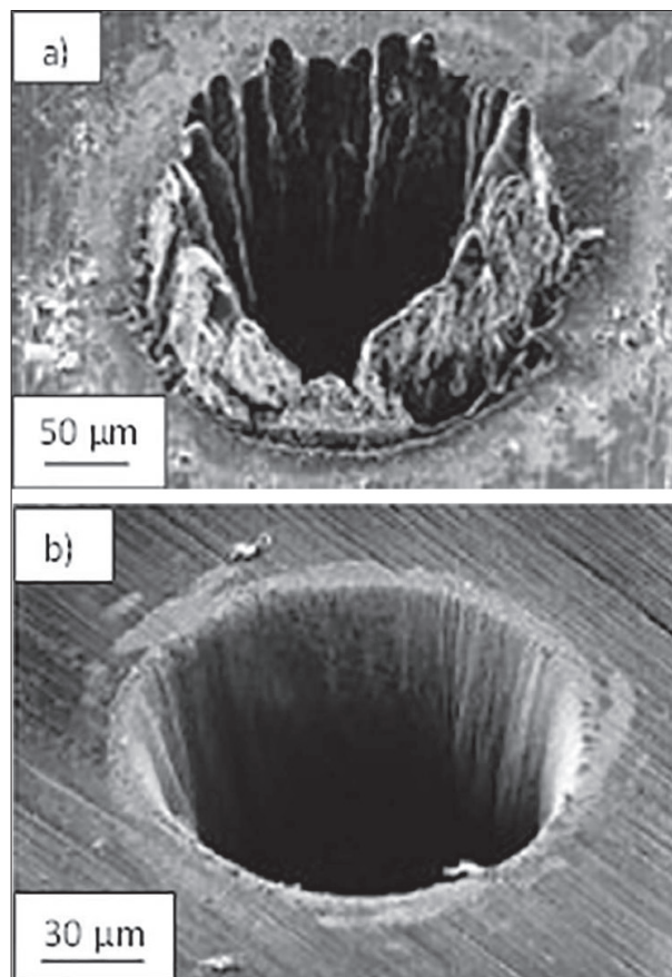
Figure 3. Craters obtained as a result of a) the femtosecond and b) the nanosecond laser radiation interaction with a steel surface [10]
