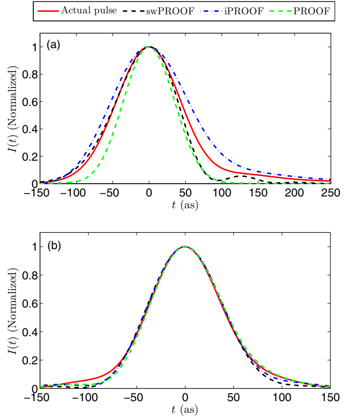
FIG. 12. (Color online) The normalized temporal intensity profile of the actual and retrieved XUV pulses for (a) case 3 and (b) case 4. The input IR parameters are the same as in Fig. 10. In the fitting procedure, E_{\text{IR}} is known.
