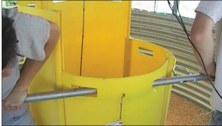
Figure 3. Grain rescue tube panels being manually inserted into the grain mass with a pipe running through the panel's hand-holds.
