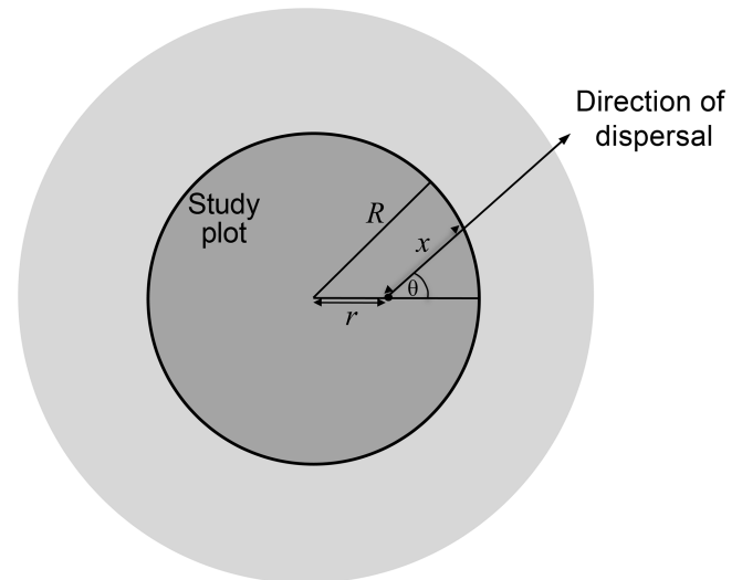
FIGURE 2. A dispersal event in direction \theta from a nest site at distance r from the center of a circular study area with radius R . The probability that a dispersal event will take the individual outside the study area is the probability that the dispersal distance is greater than distance x , where x is given by Equation 3. The dark gray area represents the study area and the surrounding light gray area represents suitable nesting habitat outside the study area.
