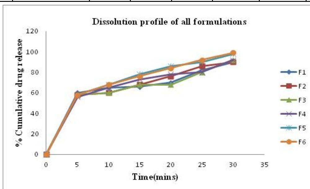
Fig. 4: Comparative dissolution profiles for F1, F2, F3, F4, F5 and F6
