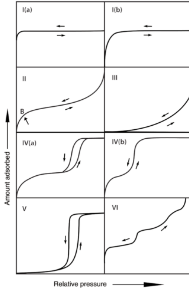
Figure 3 Isotherm types[60]
