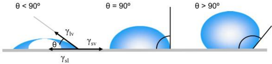
Figure 5 Illustration of the contact angle formed between a liquid and a homogenous solid surface[67]
