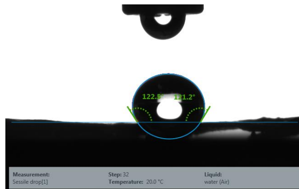
Figure 48 Contact angle of the BP
