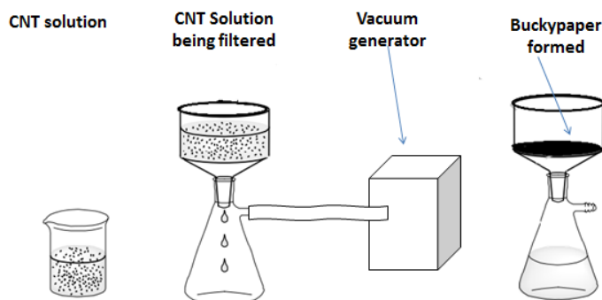
Figure 8 vacuum filtration system used
