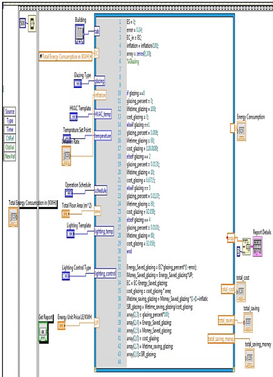
Figure (3-7) ERDSS Interactive Database savings calculation section (LabVIEW)
