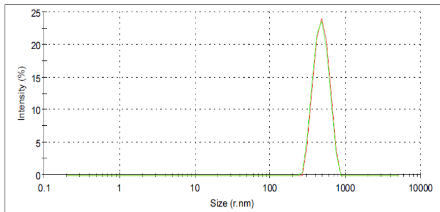
Figure (5-1) Average particle size and size distribution of the TiO 2 nanoparticles prepared by dropwise addition of DI as measured by DLS.
