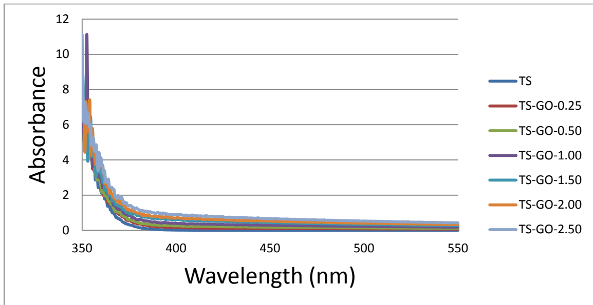
Figure (5-11) UV–Vis DRS spectra of TS-GO samples.
