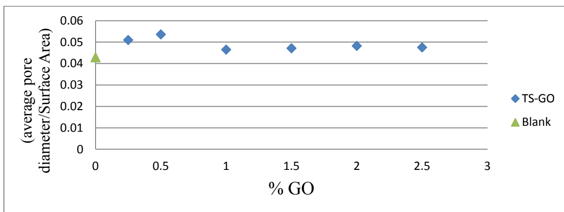
Figure (5-10) Variation of average pore diameter per surface area of TS-GO samples with percentage content of GO.
