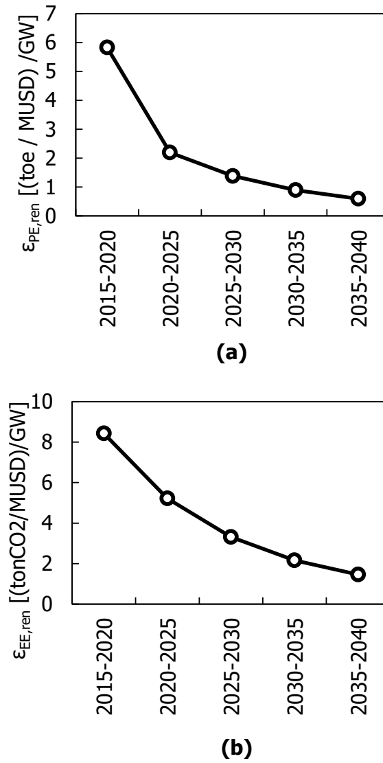
Figure 18 Potentials for reductions in energy intensity (a) per unit of renewables installed capacity and CO 2 emissions (b) per unit of renewables installed capacity.
