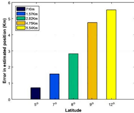
Figure 6. Error in estimated location at various latitudes.
