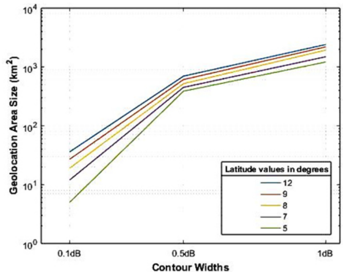
Figure 7. Geolocation area at various contour widths.
