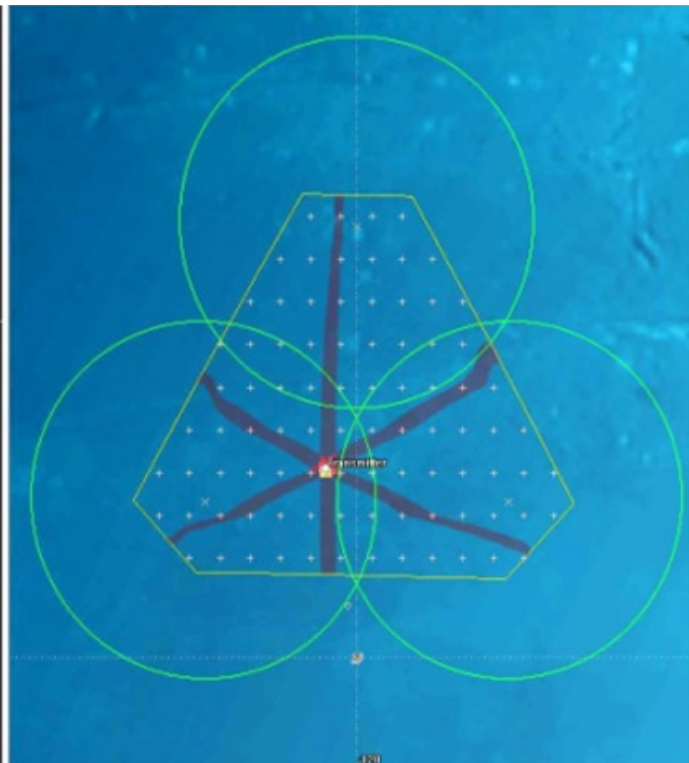
Figure 5. Intersection LOP and subsequent display at transmitter position at 50^{\circ} latitude, -1190^{\circ} longitude.
