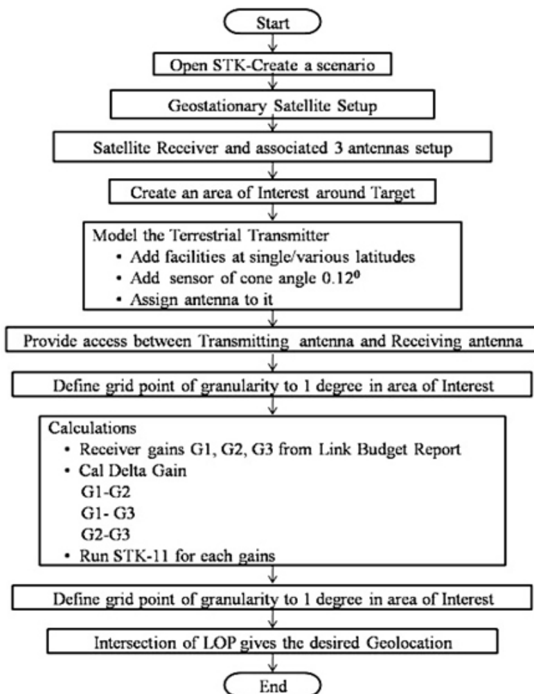
Figure 1. Flowchart for modelling of space environment using STK.
