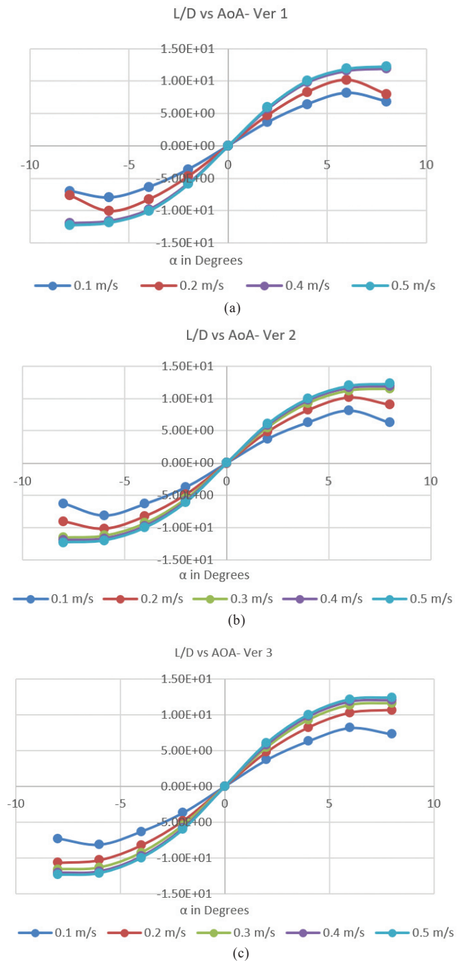
Figure 8. Lift/ Drag Ratio for three versions w.r.t \alpha (in degree) on x-axis.
