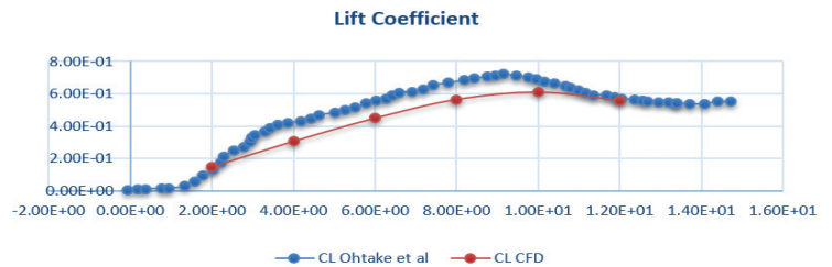
Figure 4. Lift Coefficient (on y-axis) vs AoA in degrees (on x-axis).
