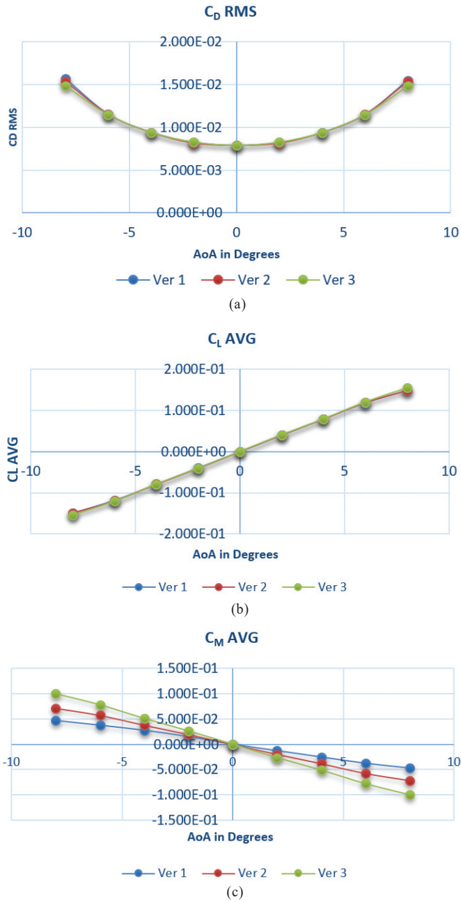
Figure 9. C_D RMS, C_L Average and C_M Average vs AoA (in Degrees) on x-axis for three versions.
