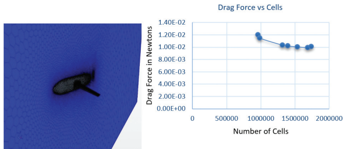
Figure 7. View showing mesh of glider, symmetry plane and grid independency study.
