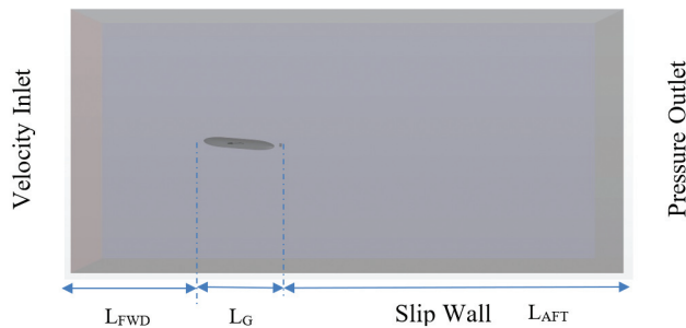
Figure 6. Domain details and boundary conditions.
