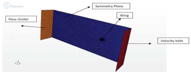
Figure 3. Boundary conditions for the study of NACA0012 wing.
