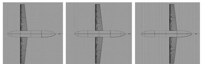
Figure 5. Three versions of the AUG with different wing position (Version 1 to 3 left to right).
