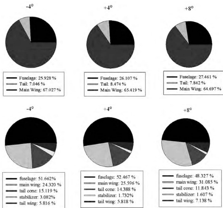
Figure 1. Lift and drag force distribution of an underwater glider 11 .
