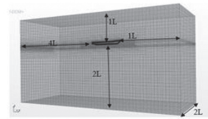
Computational domain
