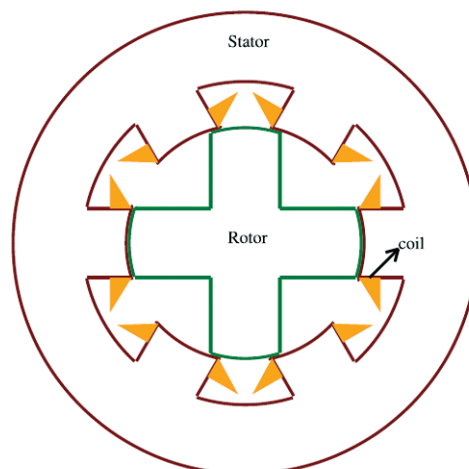
Figure 1. Construction of switched reluctance motor.
