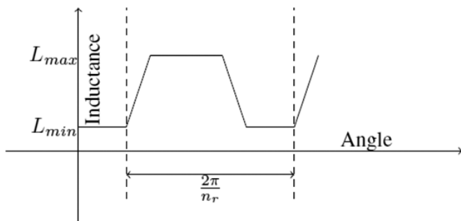
Figure 2. Typical inductance profile of SRM.
