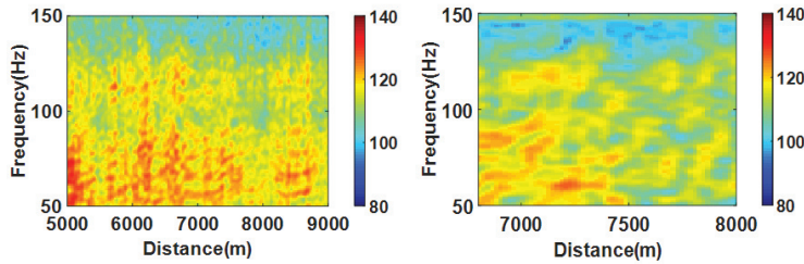
Figure 4. Range vs frequency plot of signal received level.
