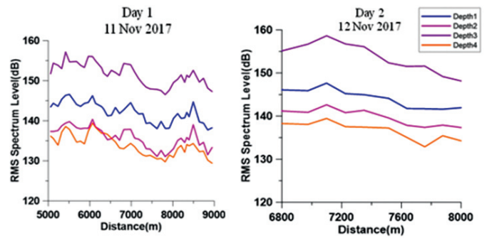
Figure 2. Range vs received rms.
