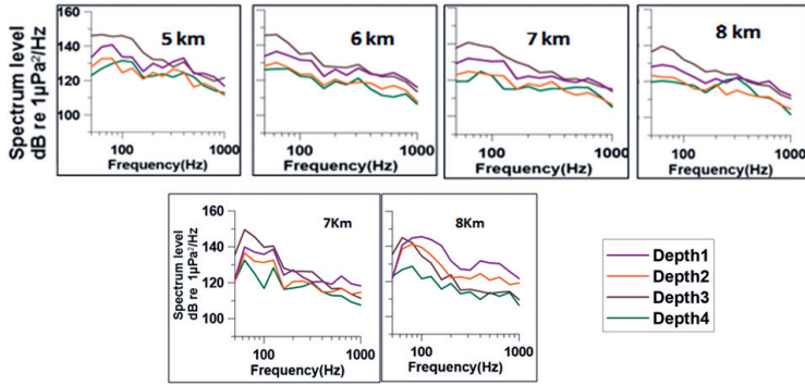
Figure 3. Spectral analysis results at typical depth, top panel for day1 and bottom panel for day2.
