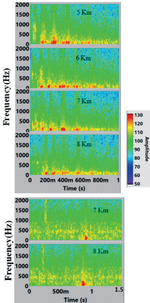
Figure 5. Spectrogram of airgun shots left panel for day-1 and right panel for day-2.
