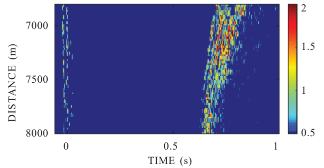
Figure 6. Acoustic intensity as arrival time-distance plot for day2.
