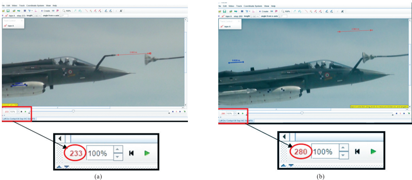
Figure 4. The screenshot of one of the data analysis using the tracker software– (a) Initial frame when the distance between drogue and probe was 2.083m. (b) Final frame when the contact was first established (closure velocity obtained was 2.46 knots).
