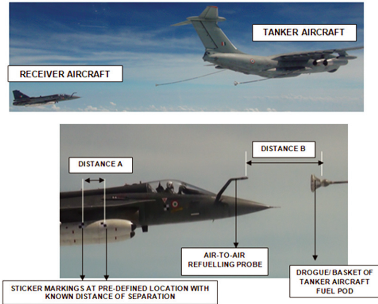
Figure 3. The snap shots showing the set-up and markings obtained from the chase aircraft.
