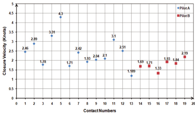
Figure 5. Graphical representation of closure velocities obtained using videographic Data.
