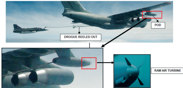
Figure 1. Ram air turbine pod reeling out the drogue basket from the tanker.
