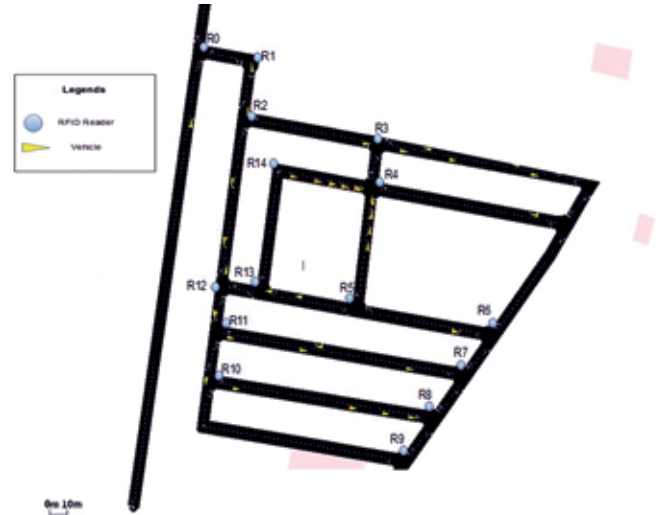
Figure 4. Simulation of RFID based vehicle detection and tracking in SUMO.
