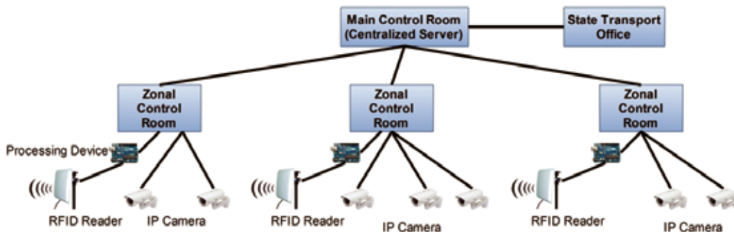
Figure 2. Configuration of data acquisition units in proposed system.
