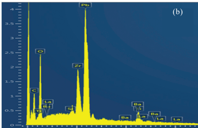
Figure 3. (a) FESEM and (b) EDAX of bulk sample.
