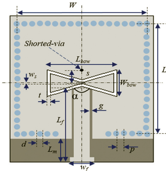
Figure 1. Antenna configuration with W=25.50 , L=24 , s=2.60 , L_{bow}=13.40 , W_{bow}=6.25 , L_m=5 , L_f=15.95 , t=0.60 , p=1.50 , g=0.4 , w_s=4.80 , w_f=0.25 , d=1 . (All dimensions are in mm).
