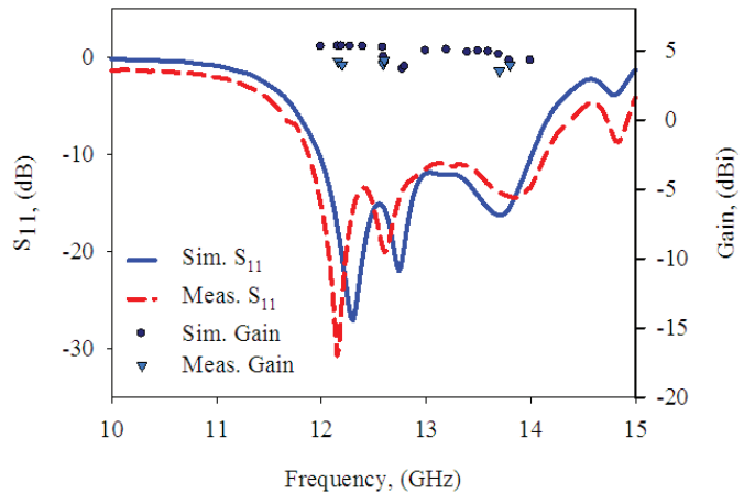
Figure 11. Comparison of simulated and measured S_{11} and gain of the proposed antenna.
