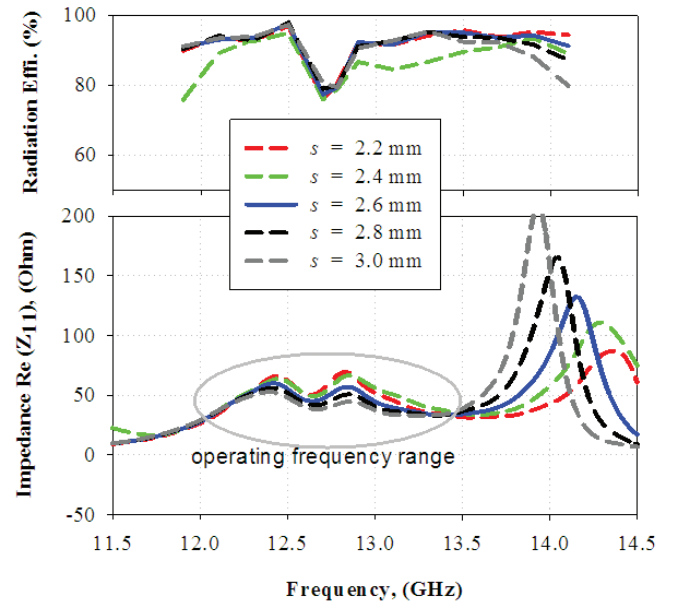
Figure 5. Effect of shorted-via on radiation efficiency and input impedance \text{Re}(Z_{11}) of antenna with change in parameter s .
