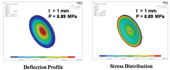
Figure 4. Deflection profile and stress distribution of diaphragm under rated load.
