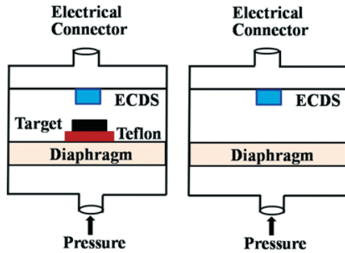
Figure 1. Pressure sensor using ECDS with and without target.
