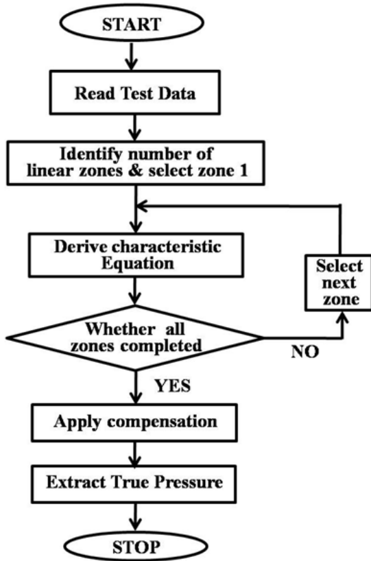
Figure 3. Flowchart illustration of target temperature compensation algorithm.
