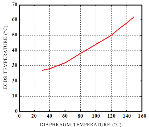
Figure 9. ECDS temperature profile.
