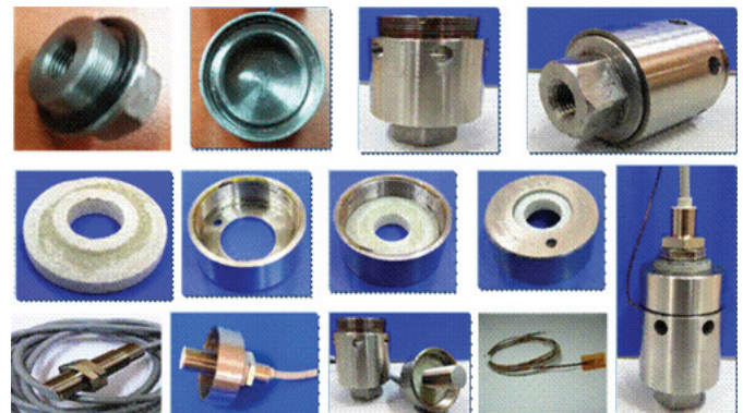
Figure 7. Various stages of assembly of pressure sensor with modified design against target temperature.
