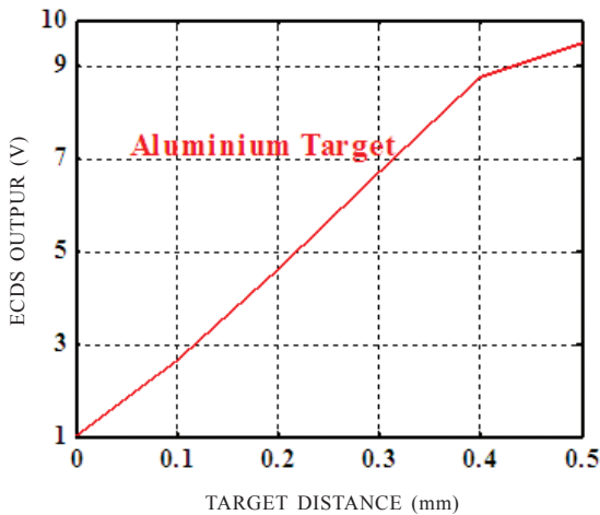
Figure 5. Calibration curves of ECDS with diaphragm and Aluminium target.
