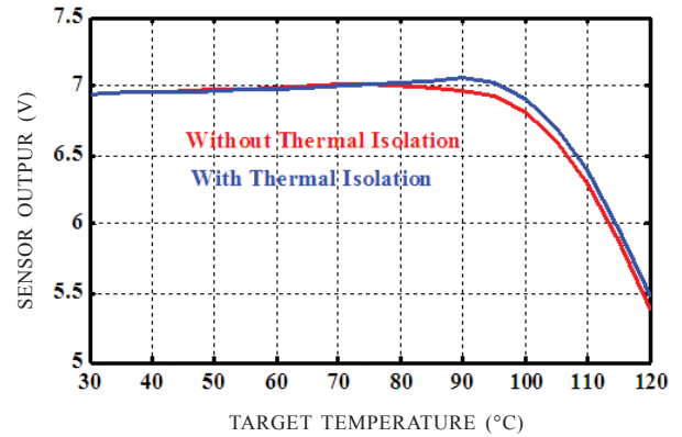
Figure 8. Comparison of target temperature effect on pressure sensor output with and without modified design.
