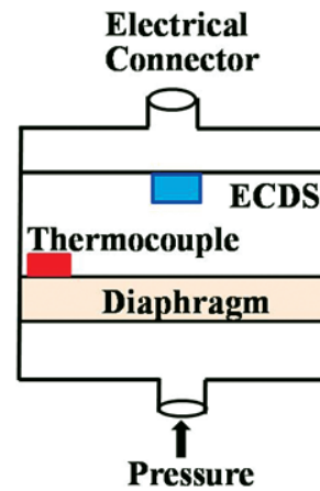
Figure 2. Scheme of proposed pressure sensor.
