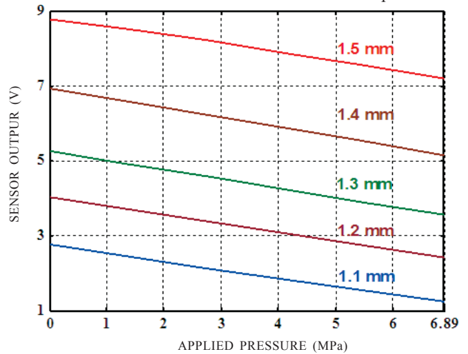
Figure 6. Calibration curves of the pressure sensor at different positions of ECDS from the diaphragm.
