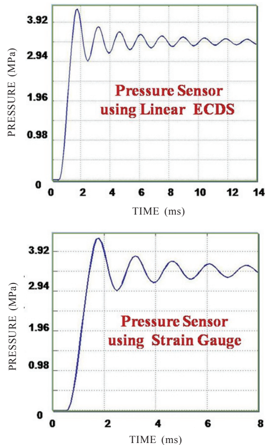
Figure 10. Step responses of pressure sensor.
