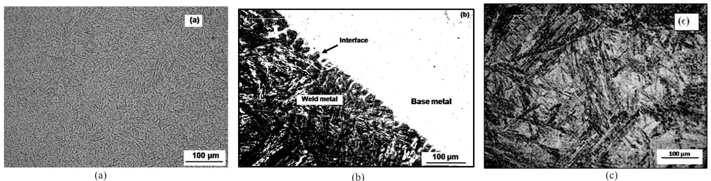
Figure 2. Microstructure of 500 °C tempered 80 mm thick Tekken specimens (a) Base metal, (b) Base metal – weldments interface, and (c) HAZ.
