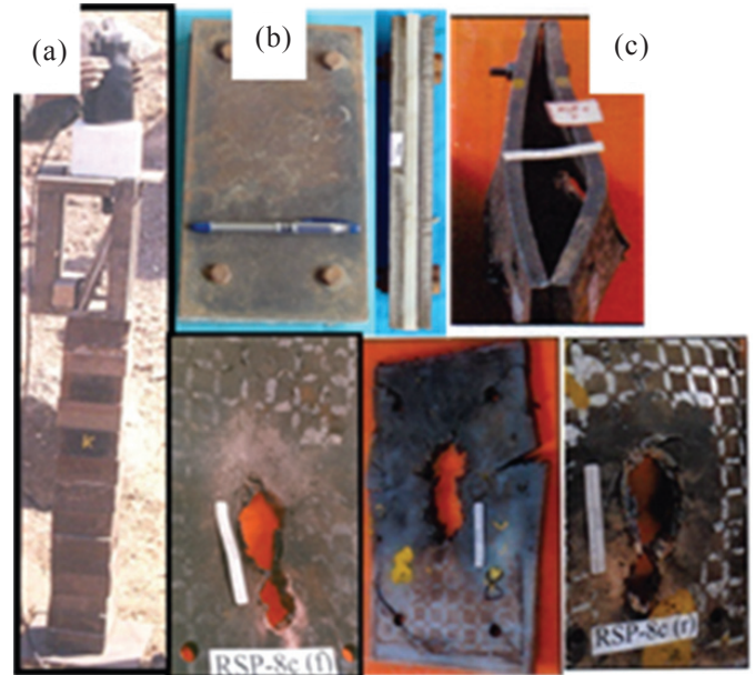
Figure 11. (a) Photographs of the test set up for firing of NERA against shaped charge warhead and bulging armour panels (b) before and (c) after penetration.
