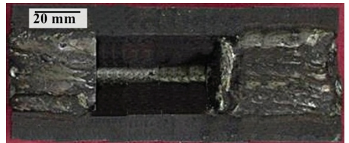
Figure 1. 80 mm Tekken specimen after welding.
