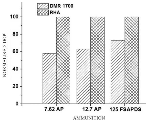
Figure 7. Ballistic performance comparison of DMR 1700 steel and RHA steel.
