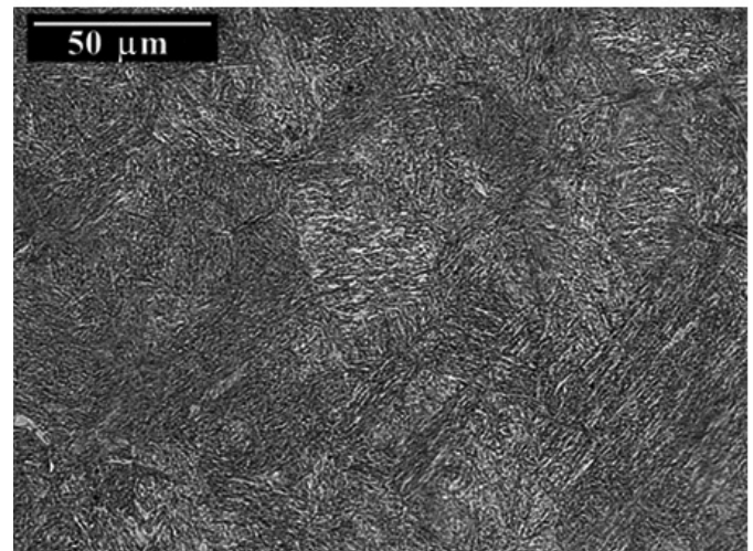
Figure 6. Optical microstructure of 50 mm DMR 1700 steel plate.
