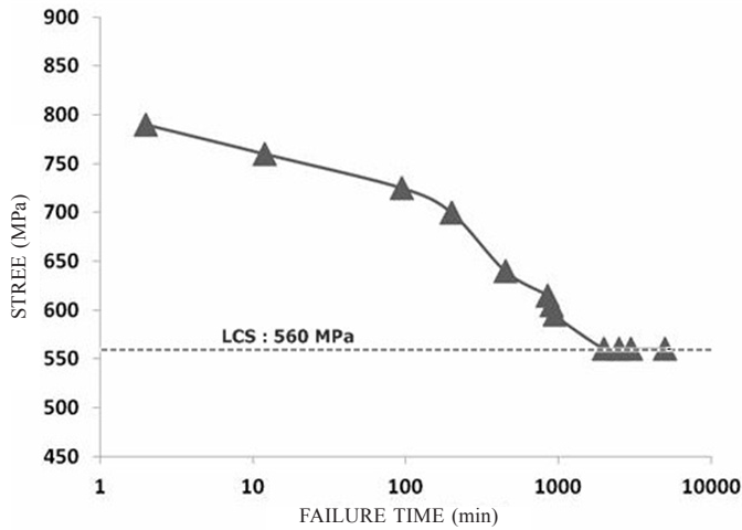
Figure 3. Stress-time curve for 500 °C tempering condition.
