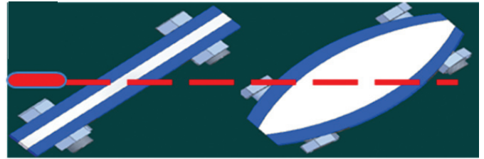
Figure 10. Working principles of non explosive reactive armour.
