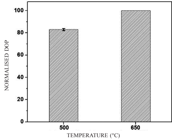
Figure 5. Large caliber ballistic evaluation results.
