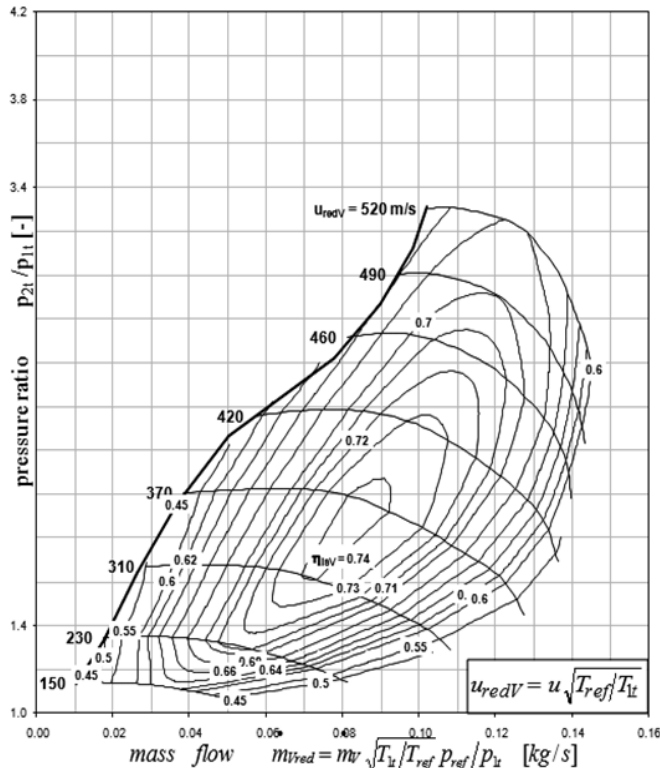
Figure 5. Compressor map.
