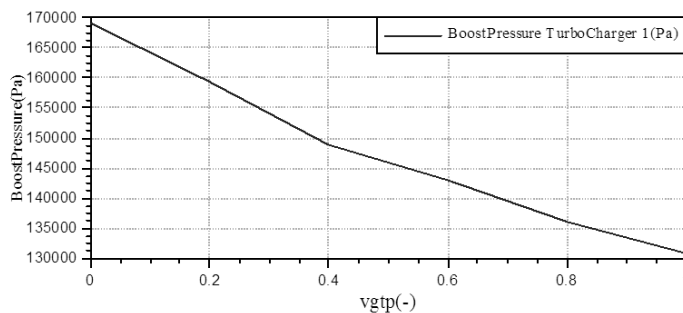
Figure 16 Effect on Boost Pressure.
