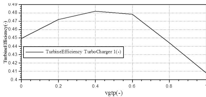
Figure 21. Effect on turbine efficiency.
