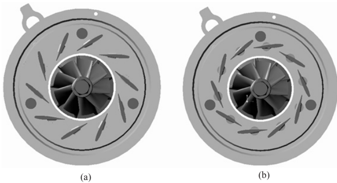
Figure 1. VGT open (a) and closed (b) nozzle blade positions.
