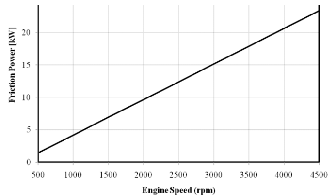
Figure 3. Friction data.
