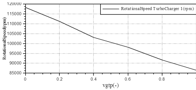
Figure 13. Effect on rotational speed of VGT.
