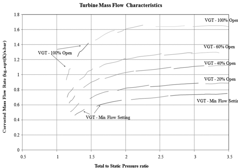
Figure 6. Turbine mass flow characteristics for different VGT positions.
