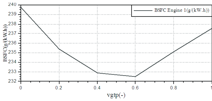
Figure 12. Effect on BSFC.
