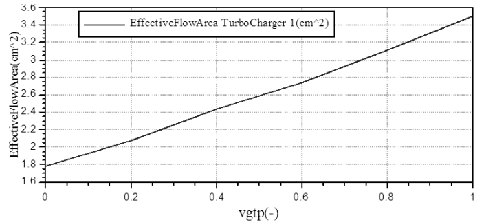
Figure 18. Effect on effective flow area.
