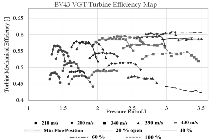
Figure 7. Turbine mechanical efficiency characteristics for different VGT positions.
