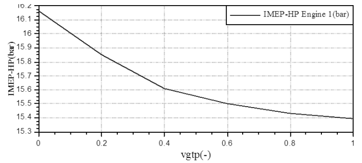
Figure 17. Effect on IMEP-HP.
