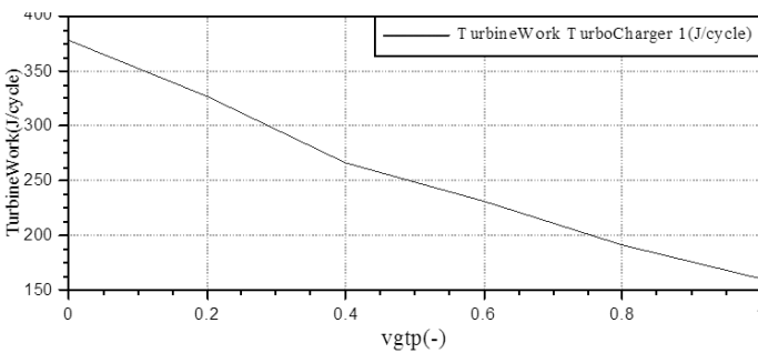
Figure 14. Effect on turbine work.
