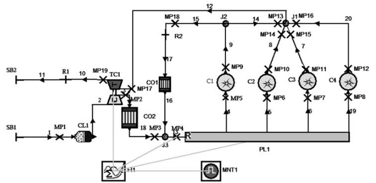
Figure 2. Thermodynamic model in AVL BOOST.
