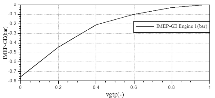
Figure 20. Effect on IMEP-GE.
