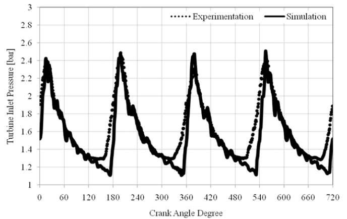
Figure 11. Turbine inlet pressure pulsations comparison.
