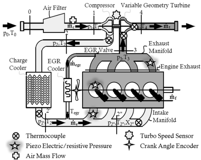
Figure 8. Instrumentation layout.
