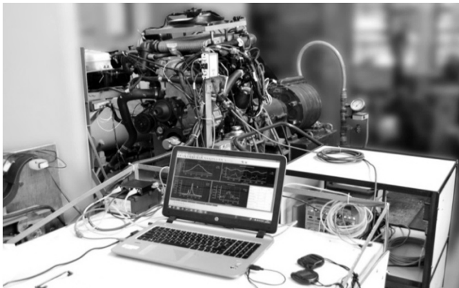
Figure 9. Experimentation setup.
