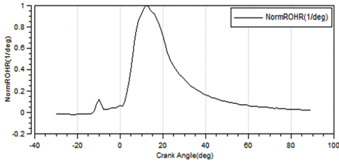
Figure 4. Combustion data as rate of heat release.
