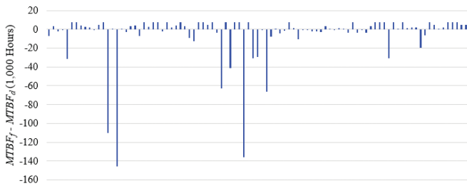
Figure 3. The distribution of MTBF Differences ( MTBF_f - MTBF_d ).
