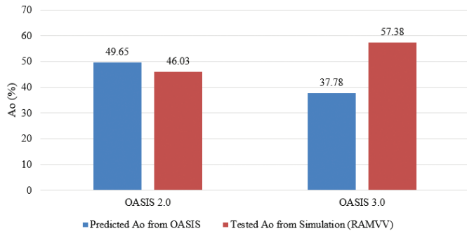
Figure 6. Results under Budget constraint (fixing B^C = 0.04 ) with modified MTBF using field data.
