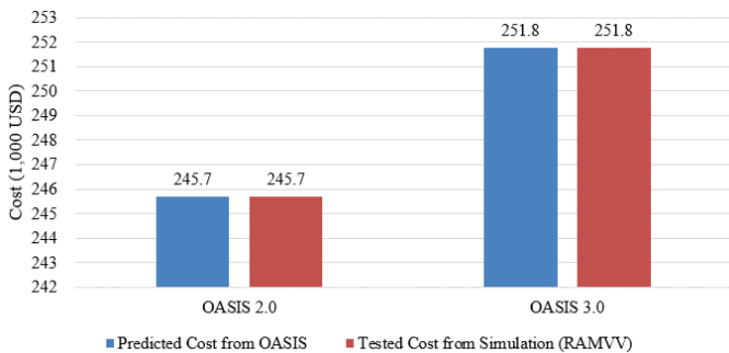
Figure 7. Results under Availability constraint ( A_o^C = 0.91 ) with modified MTBF using field data. The original cost unit was Korean Won (KRW). Exchange rate was applied for USD in Feb. 13, 2017.
