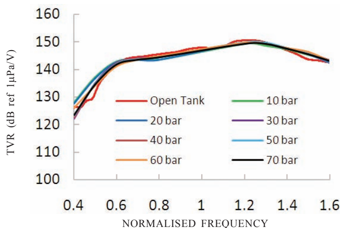
Figure 10. Measured TVR under different pressures.
