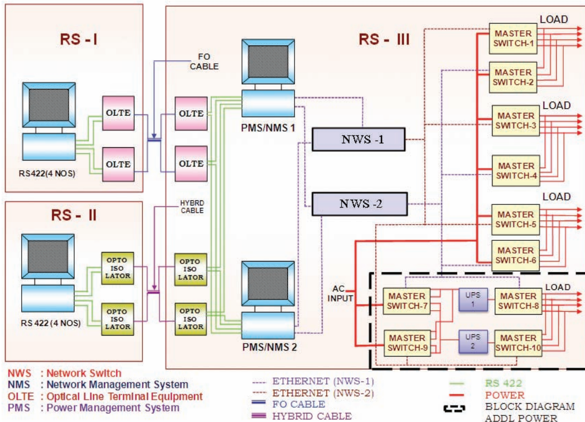
Figure 1. Power management system (PMS) and additional power requirement for underwater platform.
