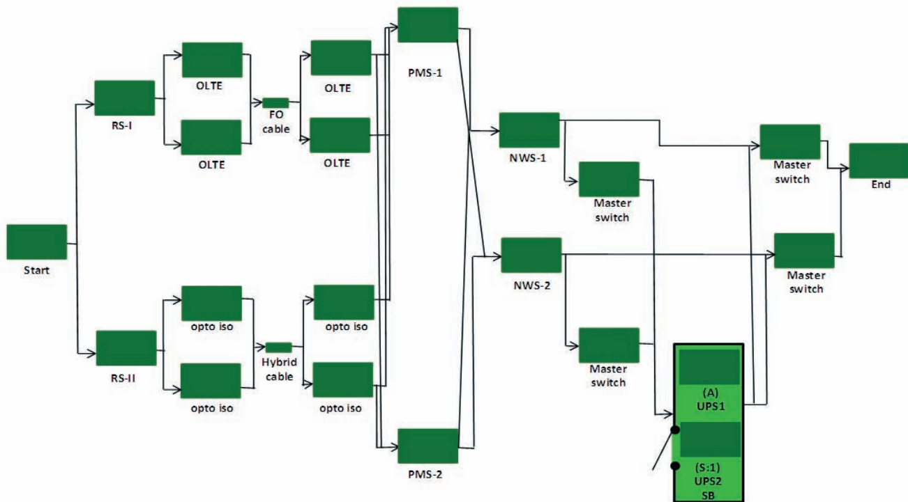
Figure 4. Reliability block diagram.
