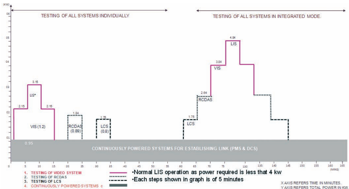
Figure 3. Power consumption cycle.
