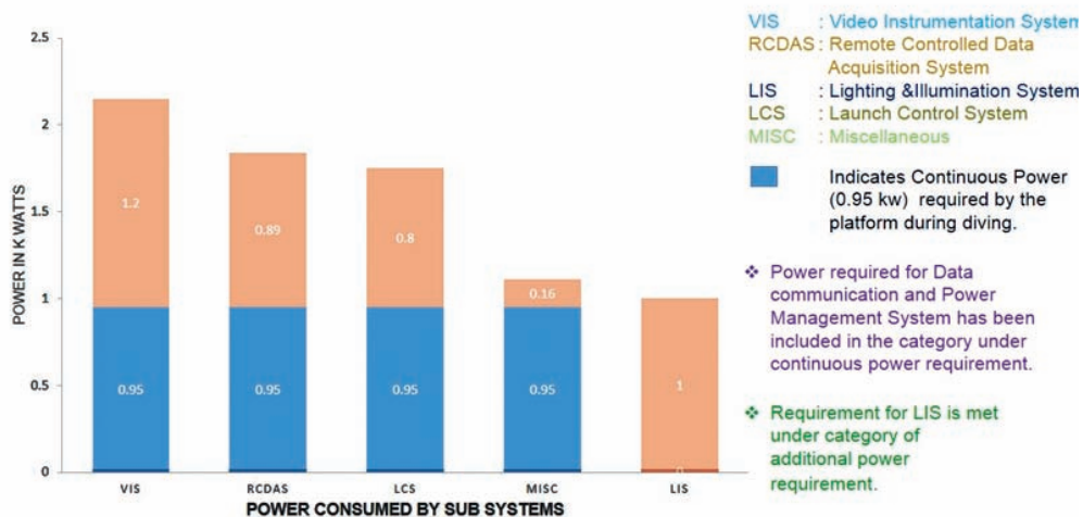
Figure 2. Power requirement managed by PMS.
