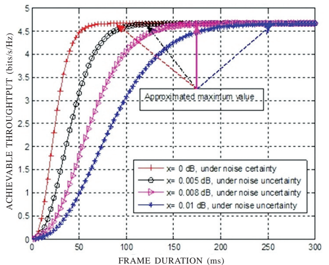
Figure 10. Analysis of SNR wall with the noise uncertainty factor x .
