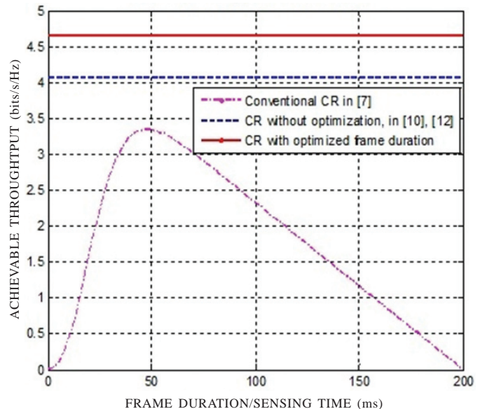
Figure 5. Variation of achieved throughput with the frame duration. Assumed SNR_p = -20 dB.
