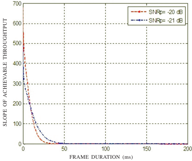
Figure 4. Variation of slope of achievable throughput with \tau .
