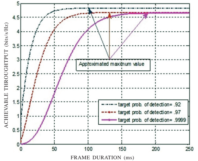
Figure 8. Achievable throughput under various values of P_d .
