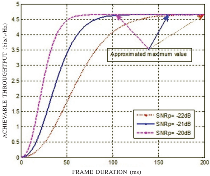
Figure 6. Achievable throughput under various values of SNR_p .
