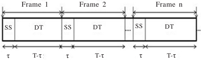
Figure 1. The conventional frame structure.
