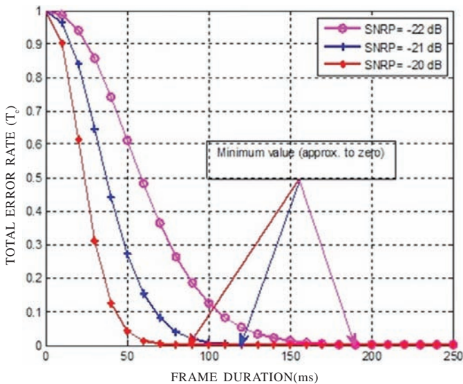
Figure 11. Achievable throughput under uncertain noise conditions.
