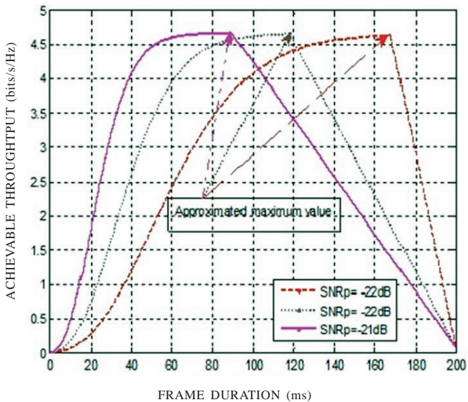
Figure 7. Achievable throughput under various values of SNR_p . It is assumed that, after time \tau^* , the PU gets activated with the probability P(H_1) = 0.3 to 0.99 .
