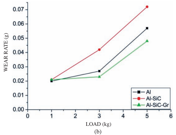
Figure 6. Variation of wear rate of different composites at sliding velocity of 1 m/s with different sliding distances: (a) 2000 m, (b) 2500 m.
