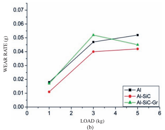
Figure 7. Variation of wear rate of different composites at sliding velocity of 1.5 m/s with different sliding distances: (a) 2000 m, (b) 2500 m.
