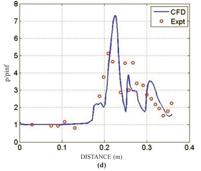
Figure 7. Ramp wall pressure comparison at various time instants for 0^\circ cowl opening (a) t = t_0 (b) t = t_0 + 1.9 ms (c) t = t_0 + 2.5 ms (d) t = t_0 + 4.5 ms.
