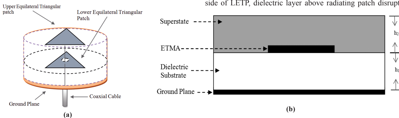
Figure 1. (a) Stacked equilateral triangular microstrip antenna, and (b) Equilateral triangular patch antenna covered with a dielectric substrate: a cross-sectional view.
