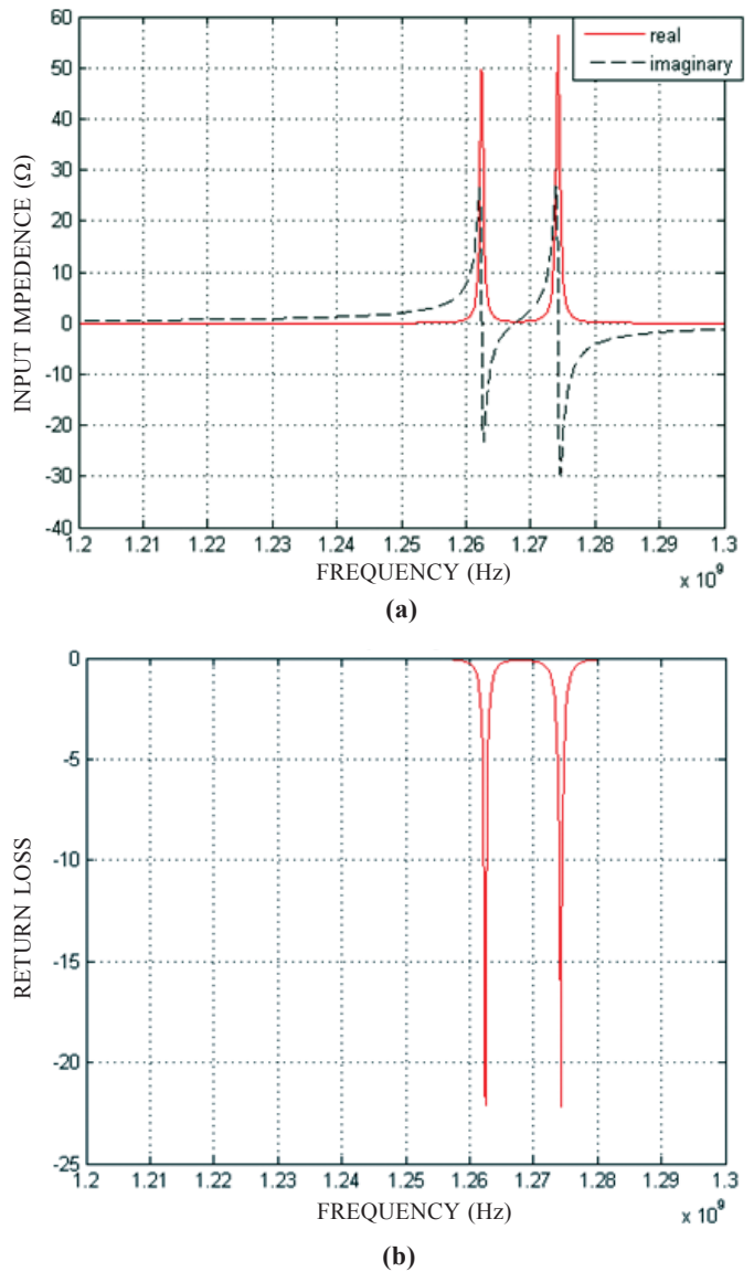
Figure 3. (a) Variation of input impedance vs frequency of stacked ETMA, and (b) Variation of return loss vs frequency of stacked ETMA.
