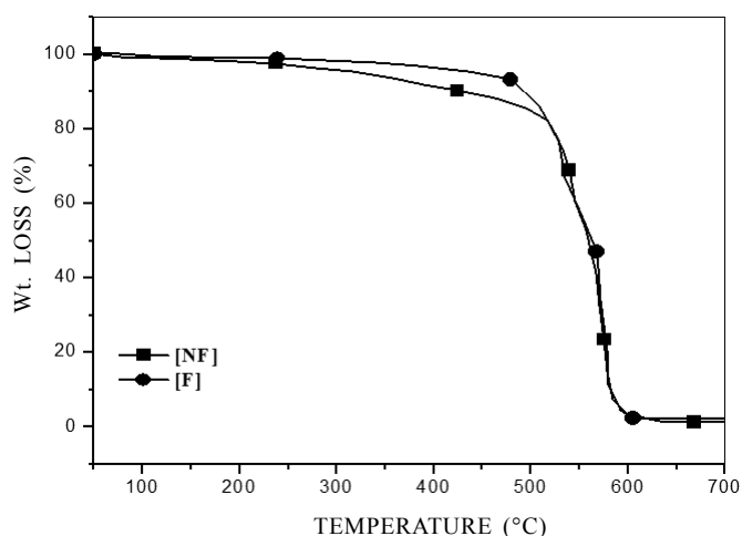
Figure 5. TG plot of the fiber, before [NF] and after [F] fluorination.
