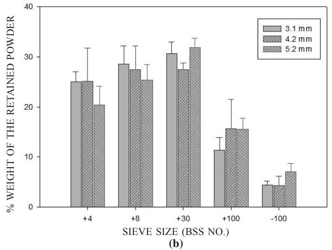
Figure 10. Particle size distribution of the impact fractured powder of (a) alumina tiles and (b) ZTA tiles with different thickness.
