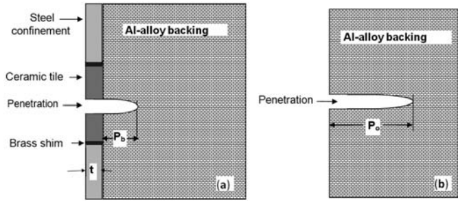
Figure 1. Schematic of DoP test configuration (a) residual DoP ( P_b ), and (b) reference DoP ( P_o ) in the backing material.
