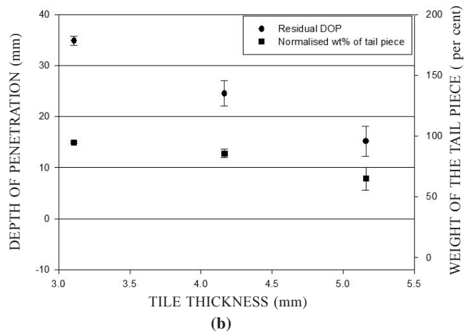
Figure 7. Residual DoP and normalised residual shot weight wrt tile thickness for (a) alumina tiles and (b) ZTA tiles.
