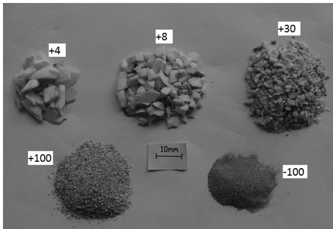
Figure 6. Impact-fractured powder (of alumina tile) retained at different sieves with BSS Nos. 4, 8, 30, and 100 are shown.
