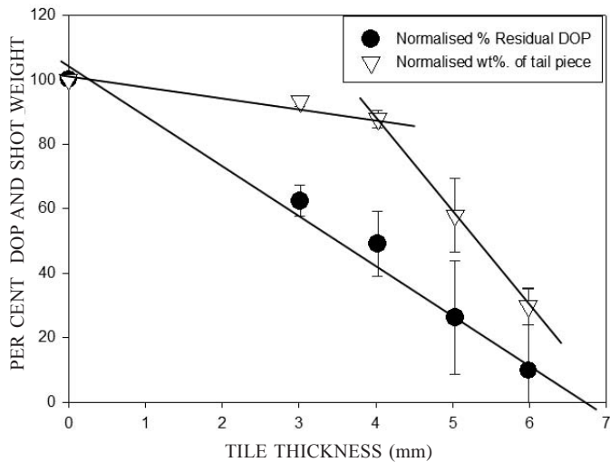
Figure 9. Normalised Residual DoP and normalised residual shot weight wrt tile thickness for alumina tiles.
