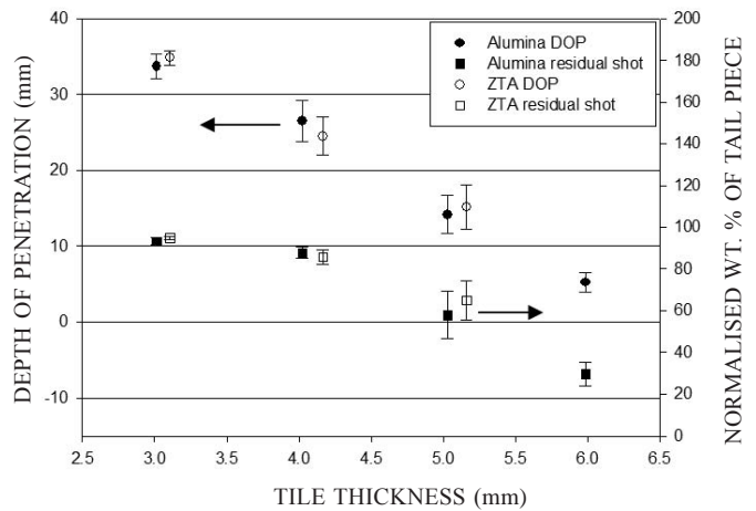
Figure 12. Comparison of DoP and shot size wrt tile thickness for alumina and ZTA tiles.
