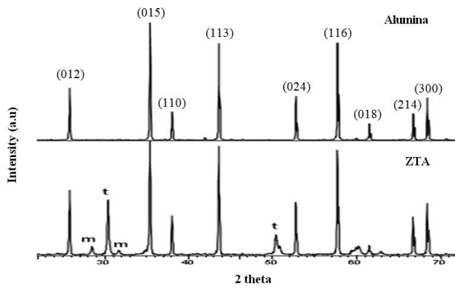
Figure 3. XRD plot of alumina and zirconia-toughened alumina (ZTA) tiles: t is tetragonal phase, m is monoclinic phase.
