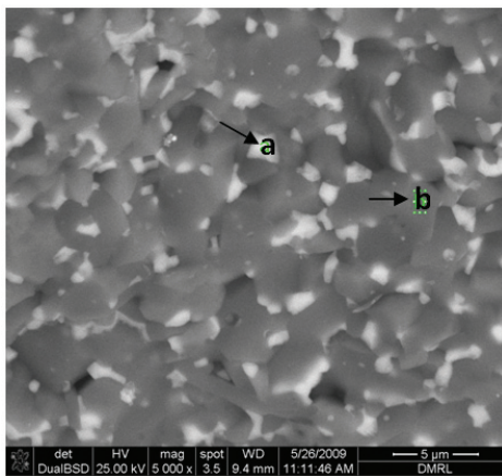
Figure 4. SEM microstructure of zirconia-toughened alumina (ZTA) shows the presence of zirconia phases dispersed in the alumina matrix; (a) Zirconia and (b) Alumina.
