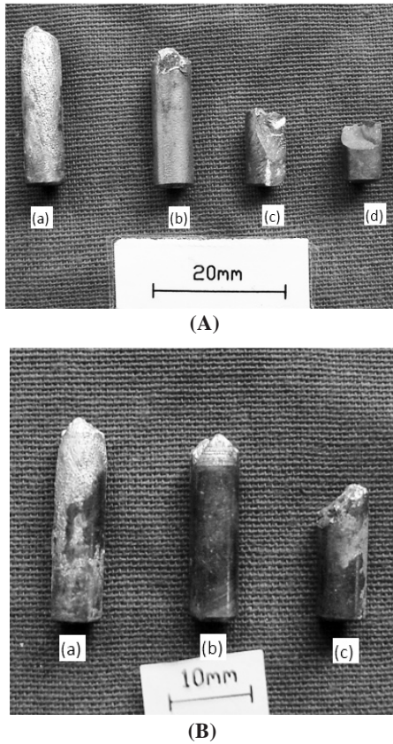
Figure 8. Tail pieces recovered after impacting ; (A) Alumina tiles with (a) 3 mm, (b) 4 mm, (c) 5 mm, and (d) 6 mm thickness, (B) ZTA tiles with (a) 3.1 mm, (b) 4.2 mm, and (c) 5.2 mm thickness, respectively.
