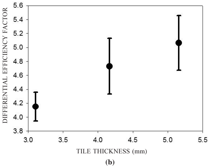
Figure 11. Variation of differential efficiency factor (DEF) wrt tile thickness for : (a) alumina tiles and (b) ZTA tiles.
