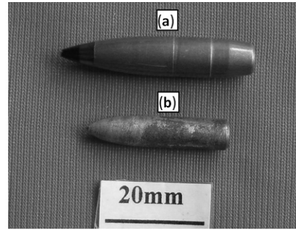
Figure 2. Photograph of the 7.62 AP shots (a) core with jacket and (b) core without jacket.
