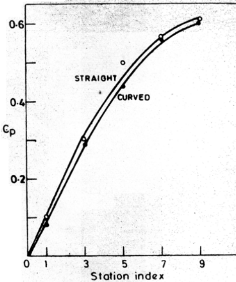
Figure 6. Comparison of pressure recovery in straight and curved diffusers ( Tu = 3.4\% ).
