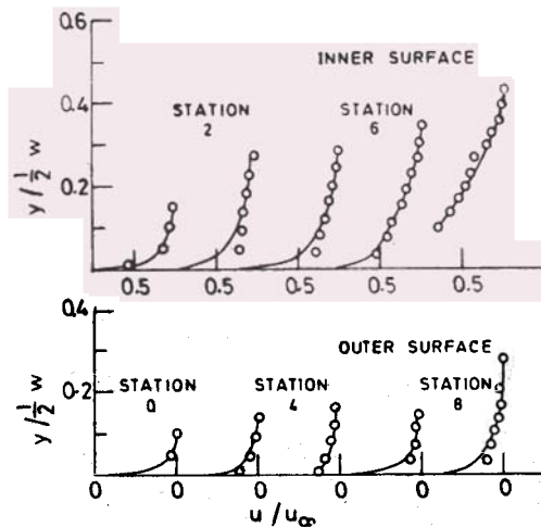
Figure 8. Boundary layer velocity profiles in a curved diffuser ( Tu = 0.7\% ).
