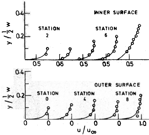
Figure 9. Boundary layer velocity profiles in a curved diffuser ( Tu = 3.4\% ).
