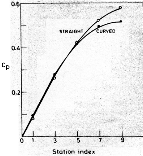
Figure 5. Comparison of pressure recovery in straight and curved diffusers ( Tu = 0.7\% ).
