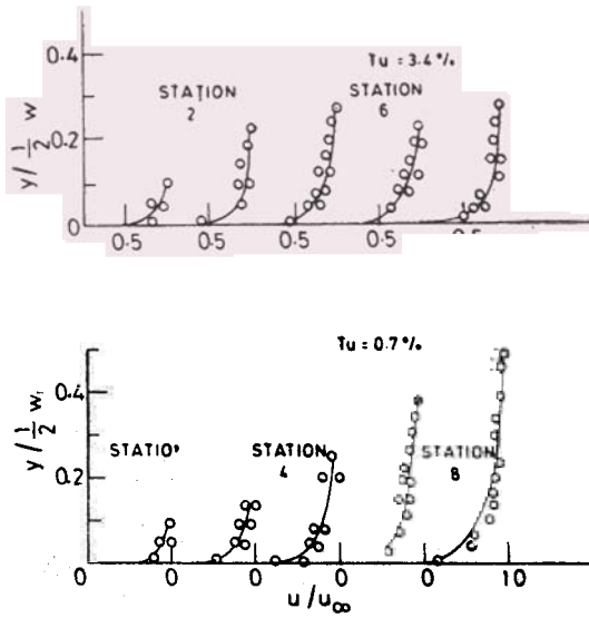
Figure 7. Boundary layer velocity profiles in a straight diffuser.
