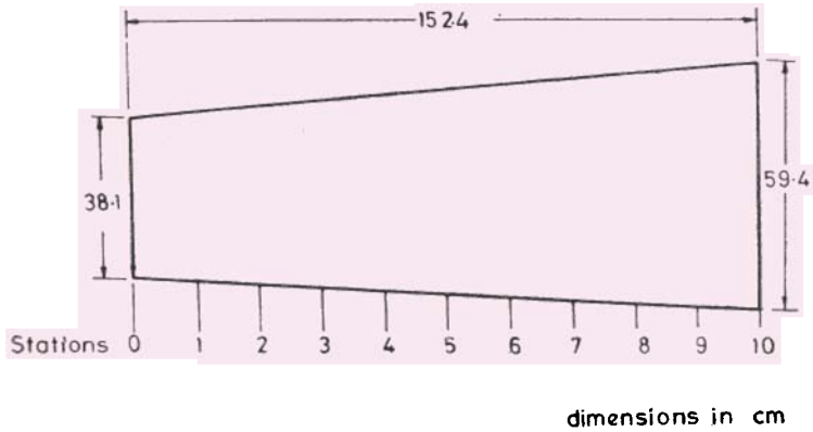
Figure 1. Two dimensional straight diffuser.
