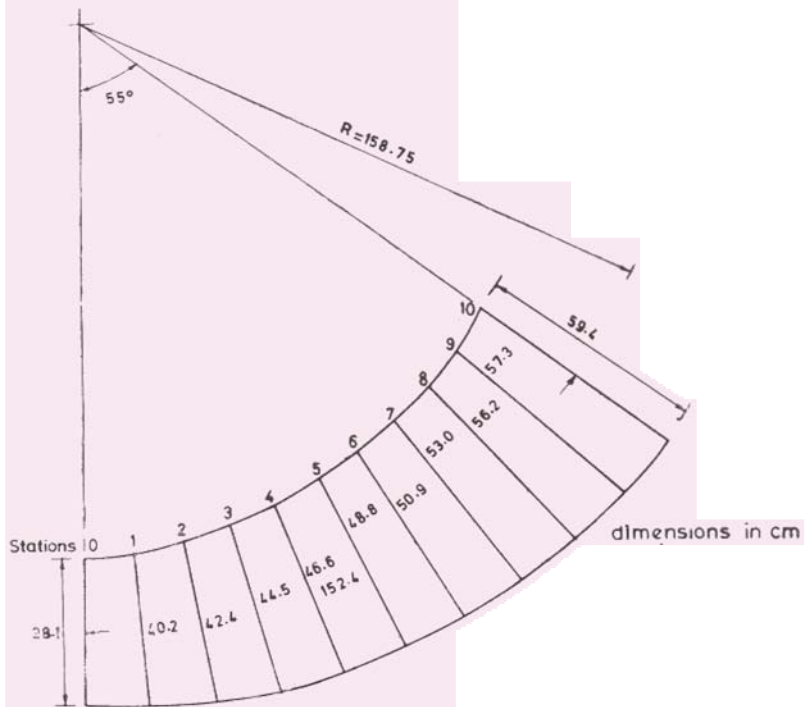
Figure 2. Two dimensional curved diffuser.
