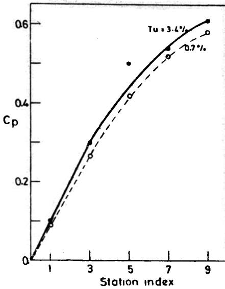
Figure 3. Pressure recovery in a straight diffuser
