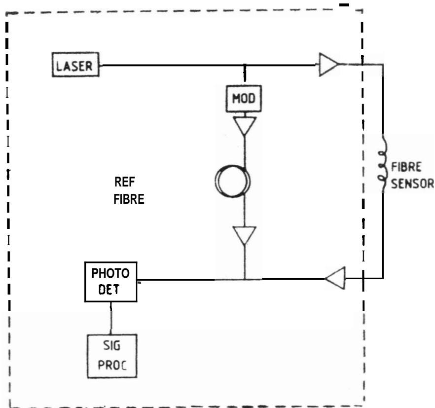
Figure 6. Fibre optic hydrophone.
