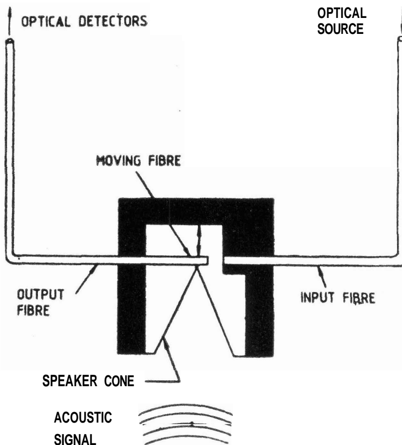
Figure 2. Multimode acoustic hydrophone.
