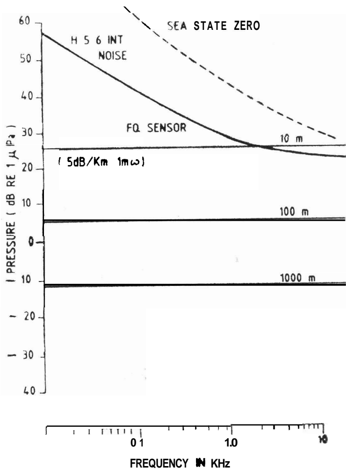
Figure 7. Quantum limited minimum detectable pressures.
