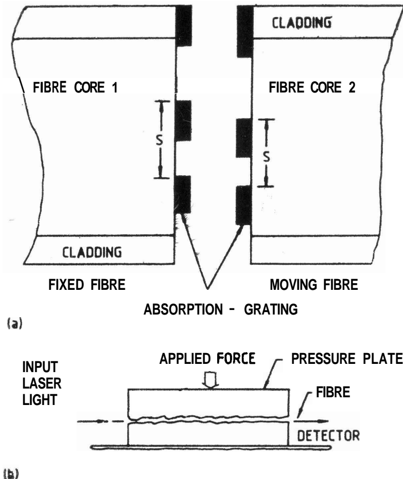
Figure 3. (a) Absorption grating, (b) Microbend hydrophone.
