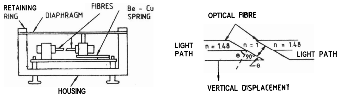
Figure 4. FTIR hydrophone.
