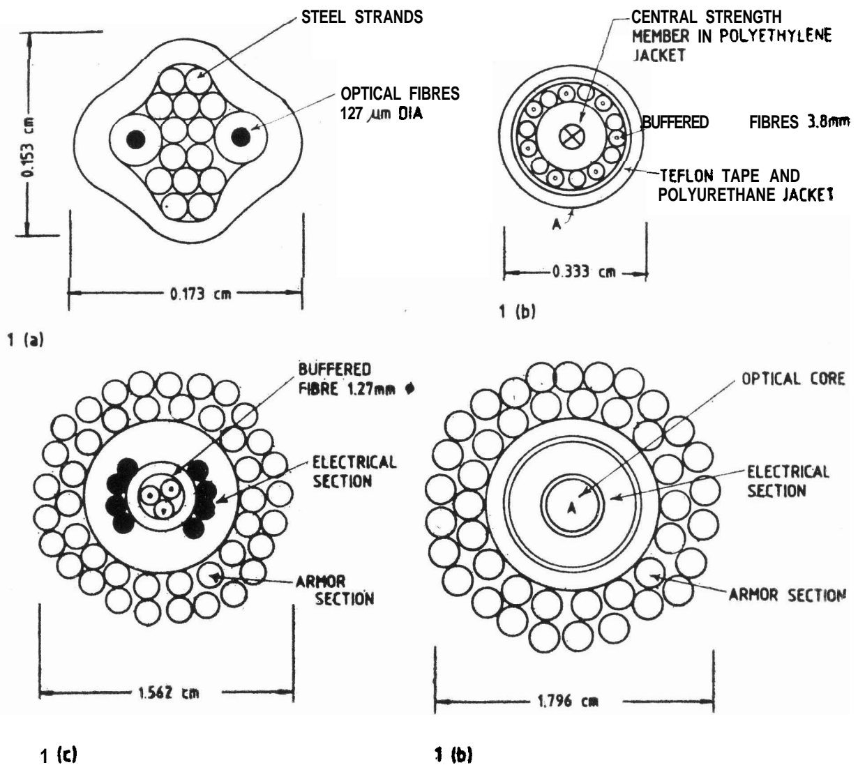
Figure 1. (a) Twin fibre cable, (b) Six fibre cable, (c) Three fibre cable.
