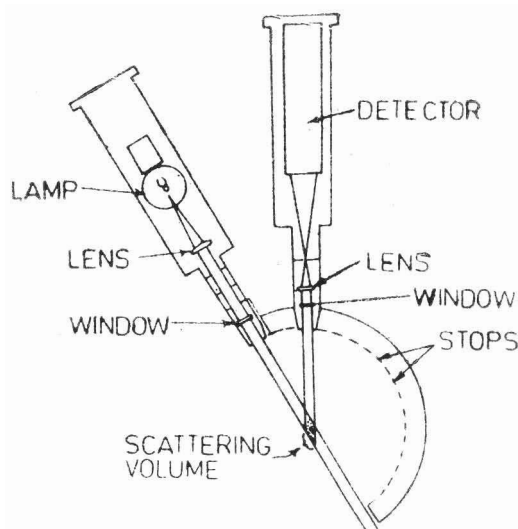
Figure 4. Scattering meter.
