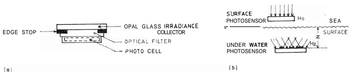
Figure 2. (a) Irradiance collector (b) Measurement of diffuse attenuation coefficient K
