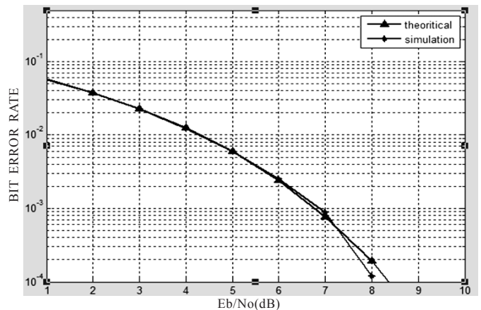
Figure 4. BER of BPSK (N= 128).
