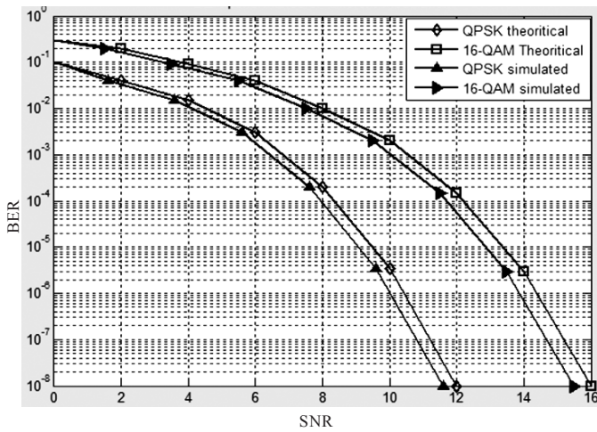
Figure 5. BER performance of OFDM with QPSK and 16-QAM.
