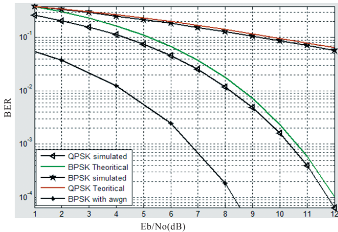
Figure 7. BPSK and QPSK for N=64 and N=128 .
