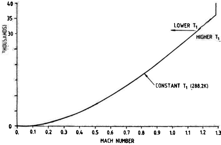
Figure 1. Mach number vs altitude at (ISA SLS Temp) T_1 = 288.2\text{K} .
