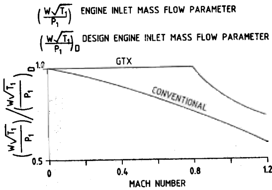
Figure 4. Estimated engine performance—ISA sea level, \bar{\tau} max dry.
