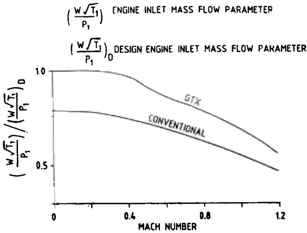
Figure 5. Estimated engine performance—ISA + 30°C sea level, max dry.
