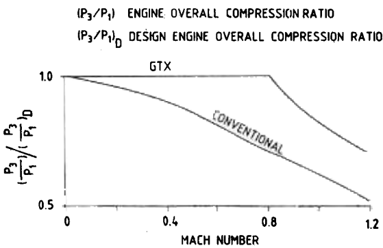
Figure 6. Estimated engine performance—ISA sea level, max dry.
