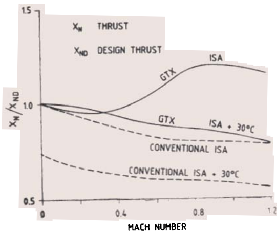
Figure 3. Estimated engine performance—sea level, max dry.
