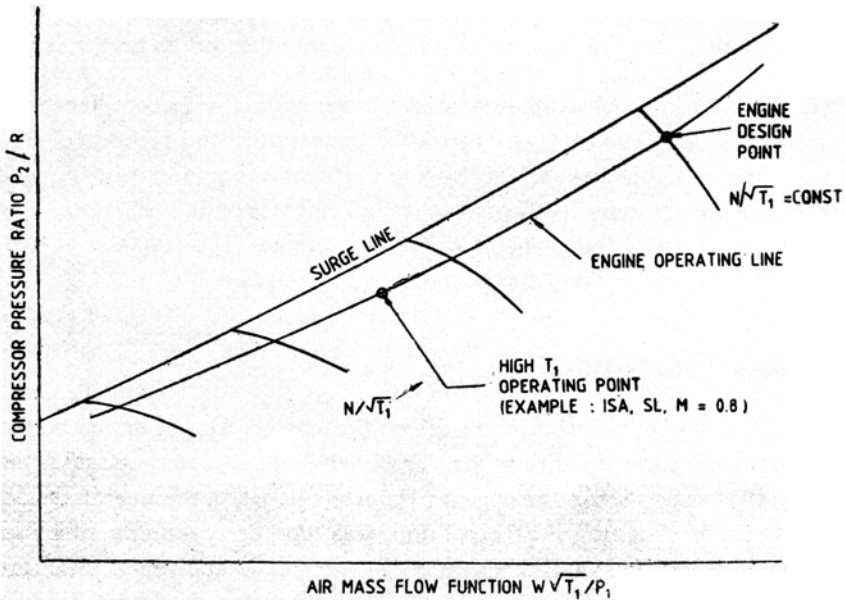
Figure 2. Compressor characteristics.
