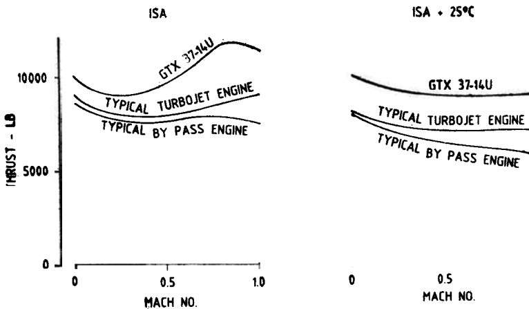
Figure 8. Comparative engine performance—sea level, max dry rating.
