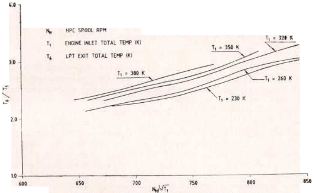
Figure 9. GTX 37-14 U estimated performance, LP turbine exit temperature.
