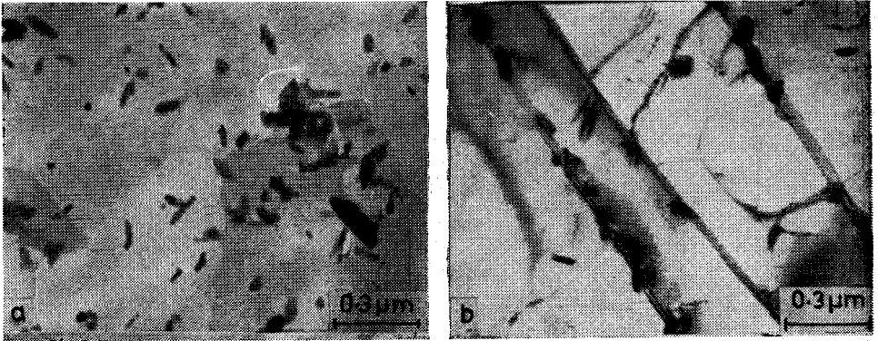
Figure 5. Transmission electron micrographs showing (a) a more homogeneous distribution of silicides in thermomechanically treated specimen and (b) silicide precipitation predominantly along the interplatelet boundaries in thermally treated (WQ-A2) specimen-Alloy IMI 685.
