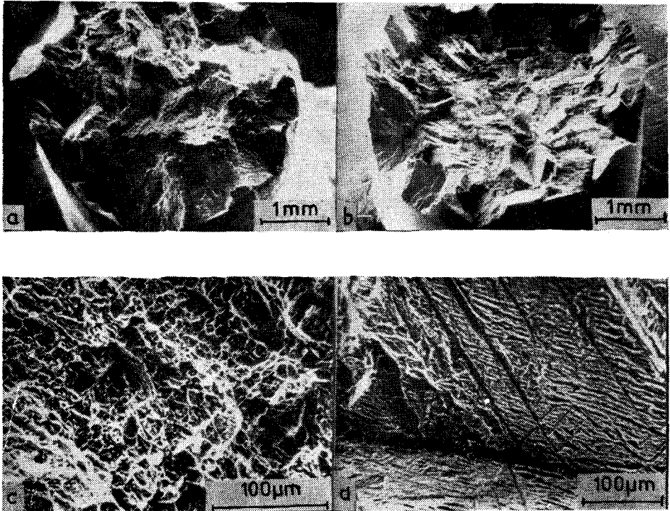
Figure 6. Alloy IMI 685 : Scanning electron fractographs showing (a) and (b) fracture surfaces of unaged and aged specimens respectively, (c) and (d) equiaxed dimples and fluted features in the central regions of the fracture surfaces of the unaged and aged specimens respectively.
