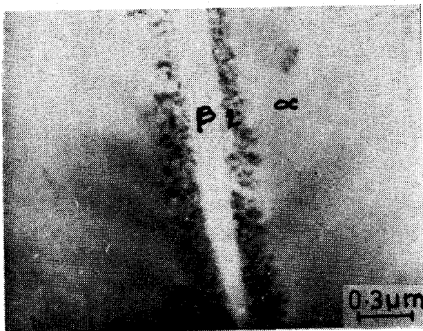
Figure 1. Transmission electron micrograph showing absence of silicide precipitates in FC-A condition in alloy IMI 685.
