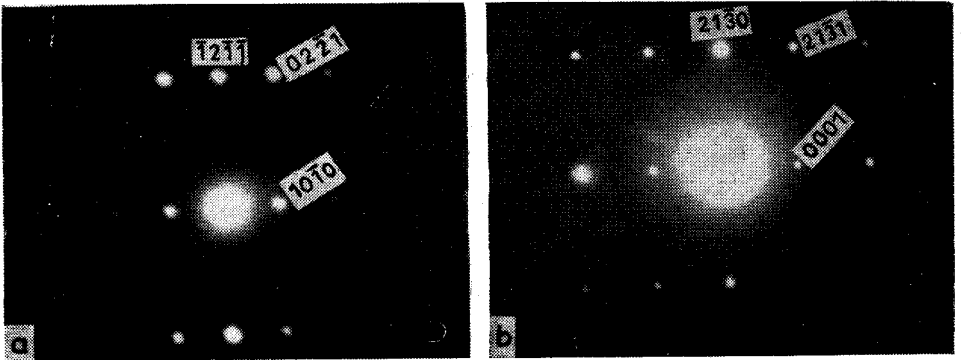
Figure 4. Selected area diffraction patterns from the S_2 silicide phase in alloy VT-9 with (a) B = [\bar{1}\bar{2}16] and (b) B = [4\bar{5}10] .
