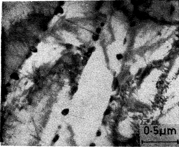
Figure 2. Transmission electron micrograph showing coarse silicide precipitates predominantly at the platelet interfaces in WQ-A3 condition-Alloy IMI 685.
