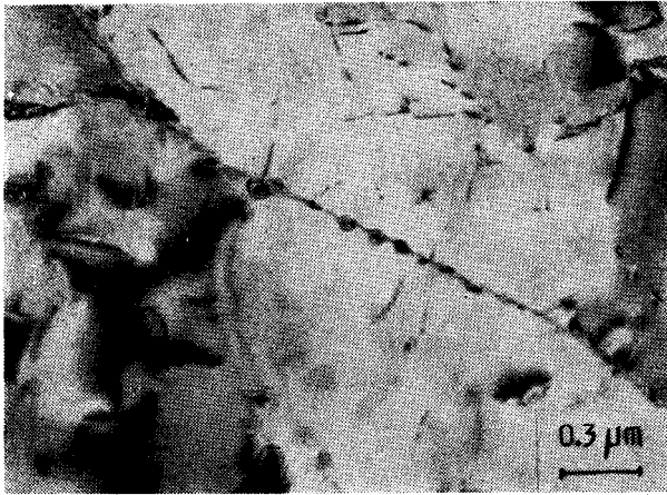
Figure 3. Alloy IMI 829 : Transmission electron micrograph showing silicide precipitates on aging at 898 K for 24 h, after solution treating in \beta at 1273 K for 1 hr followed by water quenching (Sridhar, et al 17 ).
