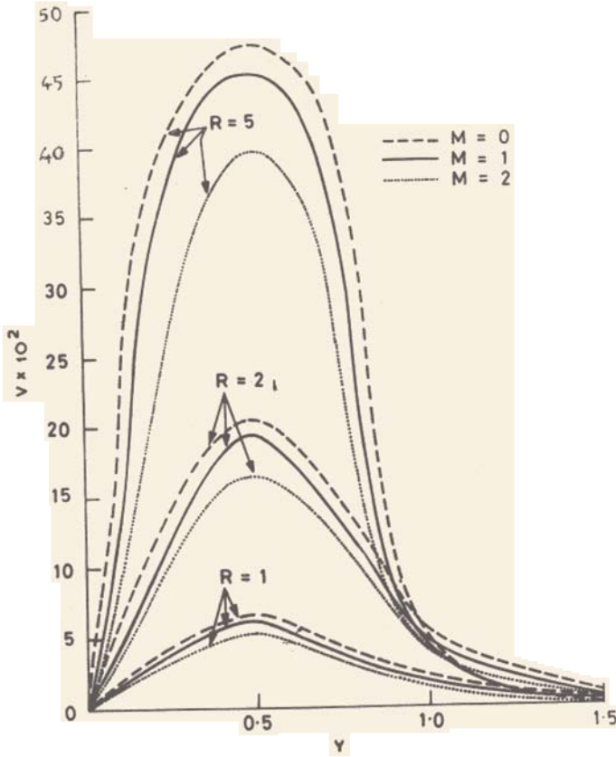
Figure 2. V(y) versus y for P=0.71 , E=0.001 and G=5 .
