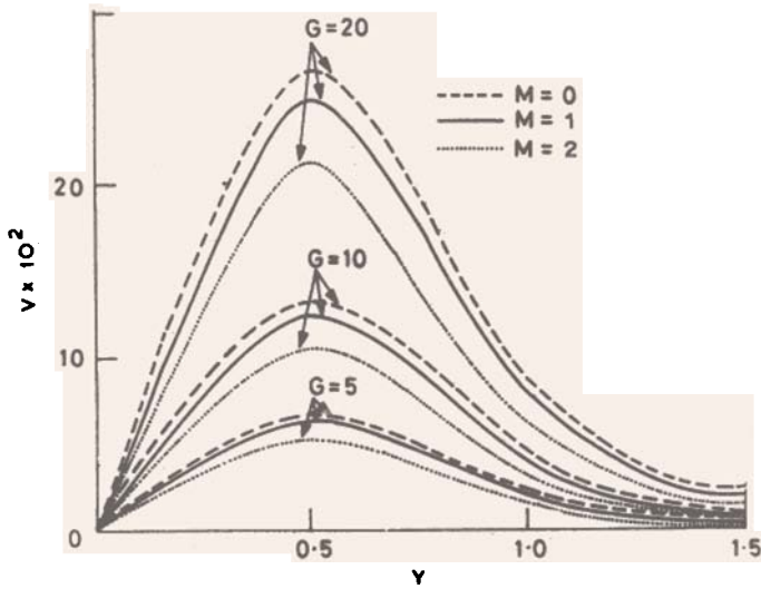
Figure 1. V(y) versus y for P=0.71 , E=0.001 and R=1 .
