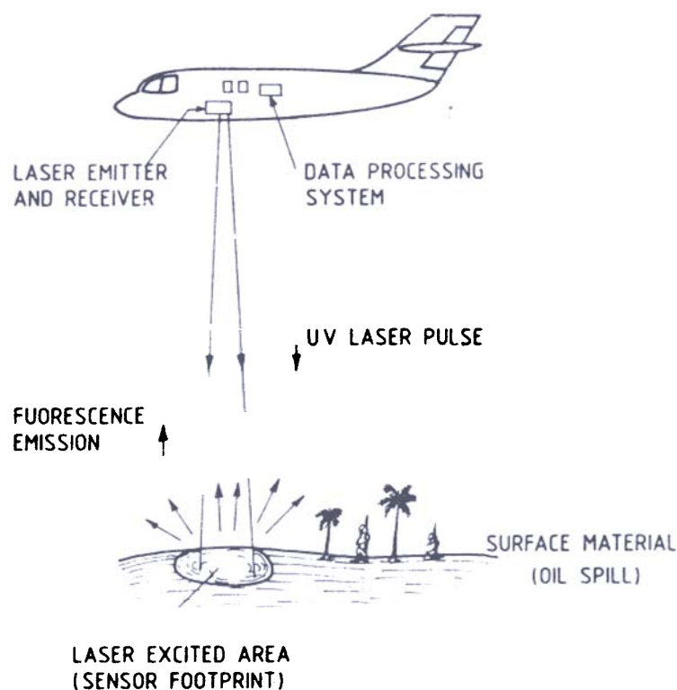
Figure Principle of airborne laser fluorosensing system.
