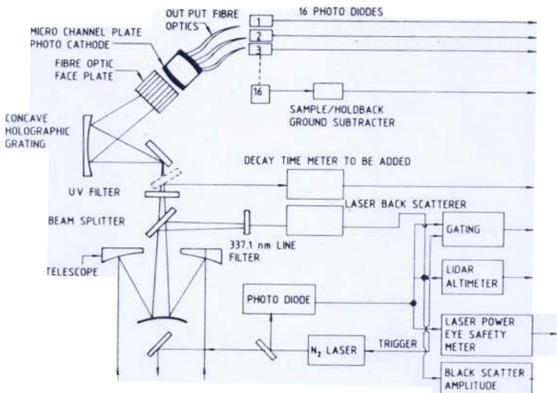
Figure 3. Schematic diagram of LF with only major electrooptic components
