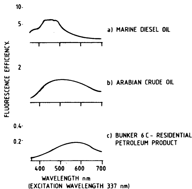
Figure 2. Fluorescence spectra of oils.
