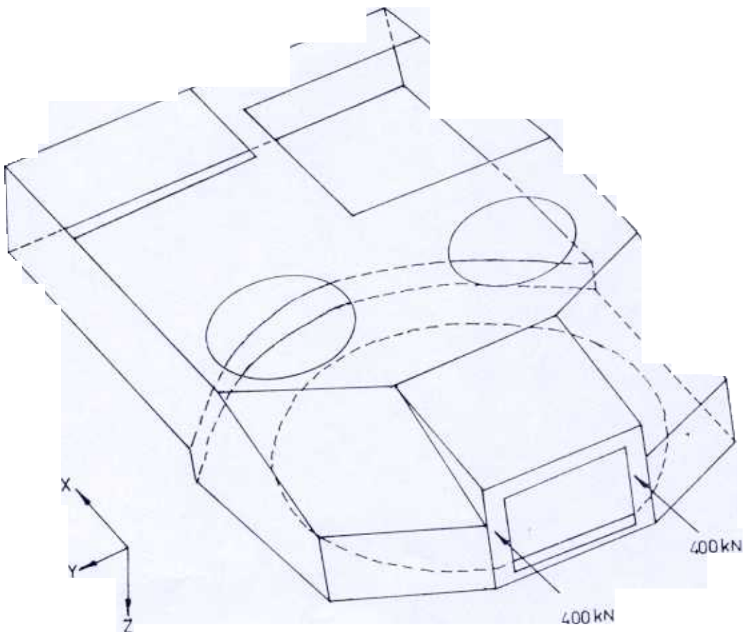
Figure 1. Pictorial view of turret.
