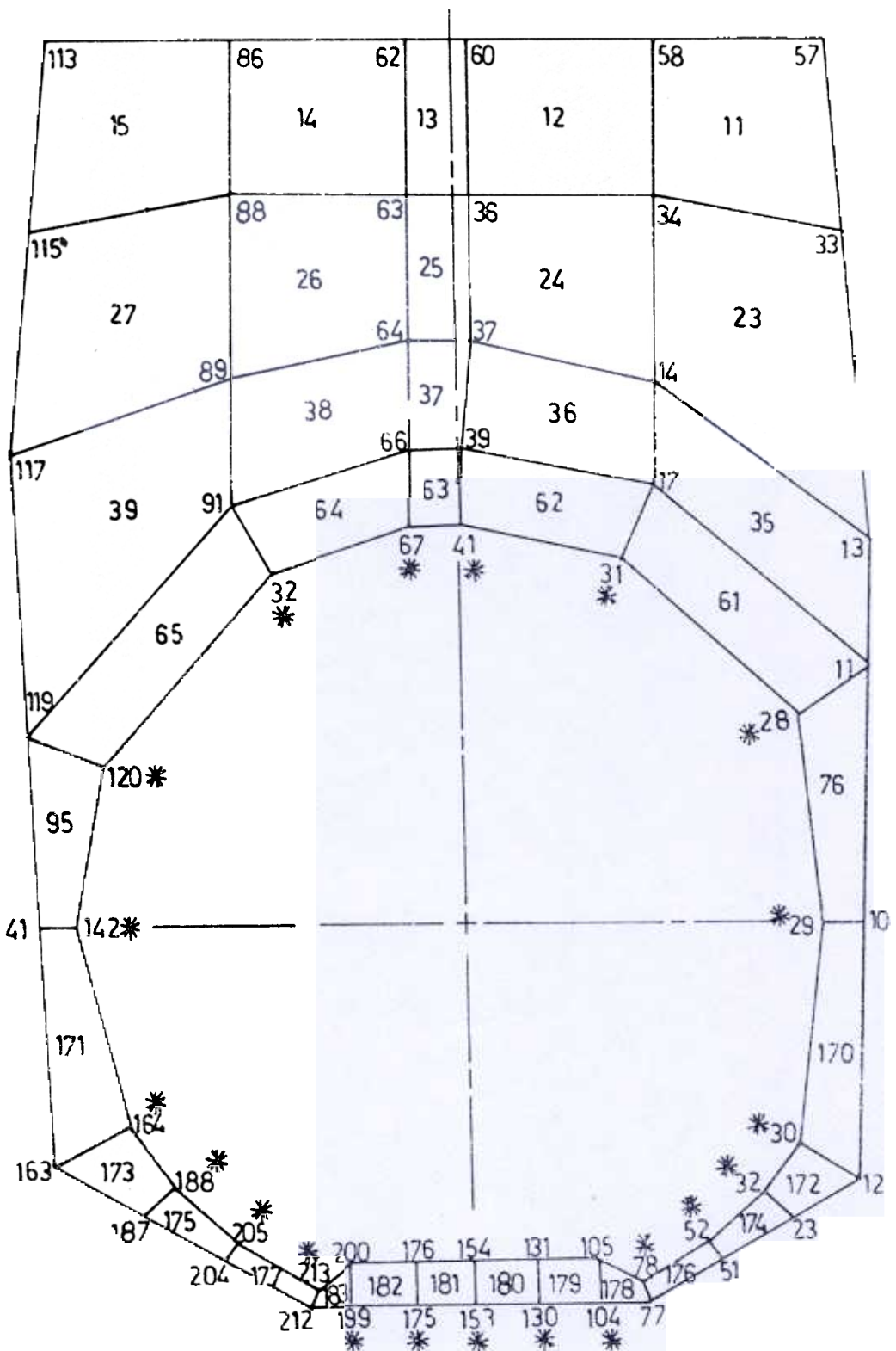
Figure 3. Turret discretization (bottom plate).
