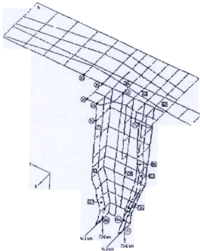
Figure 8. Graphic generated view of elevating cylinder mounting bracket.
