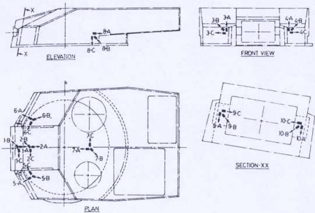
Figure 5. Strain gauge locations on turret model.
