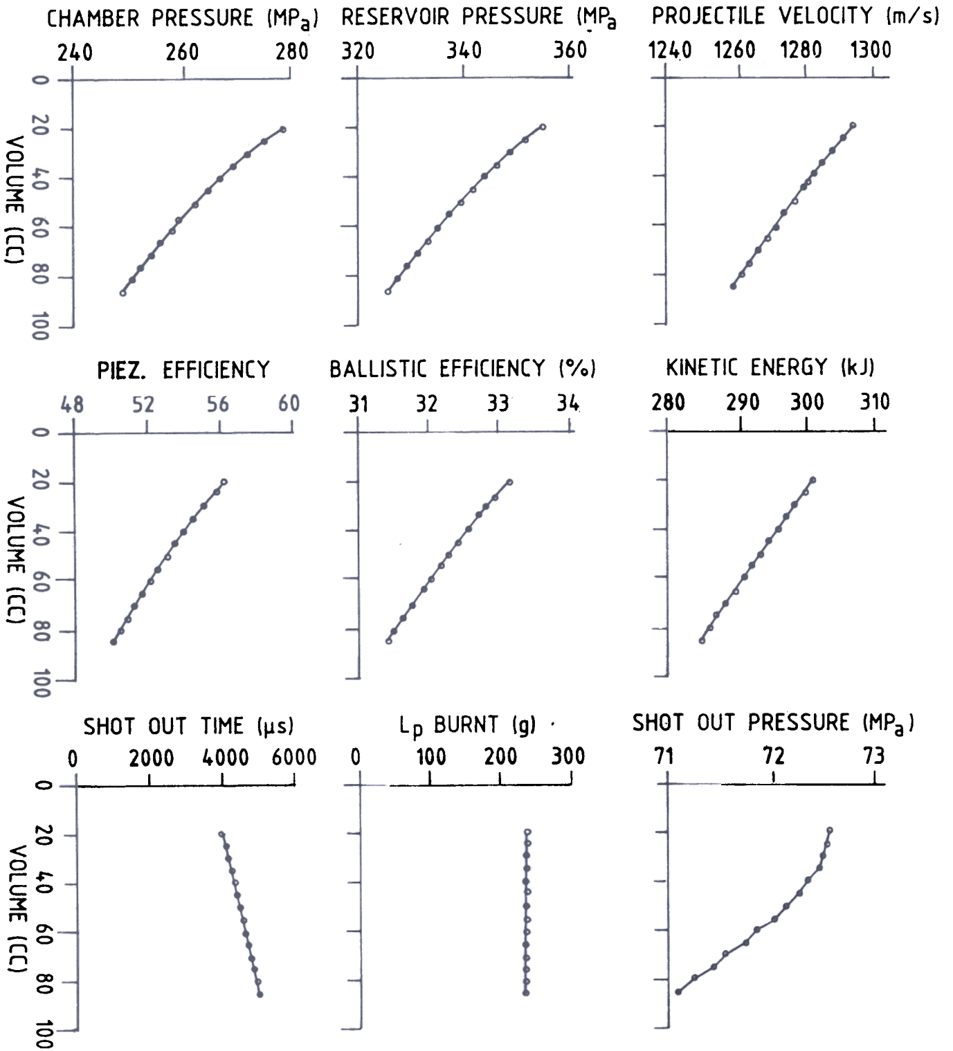
Figure Parametric study for the effect of gun performance with variation in the initial volume of the combustion chamber.
