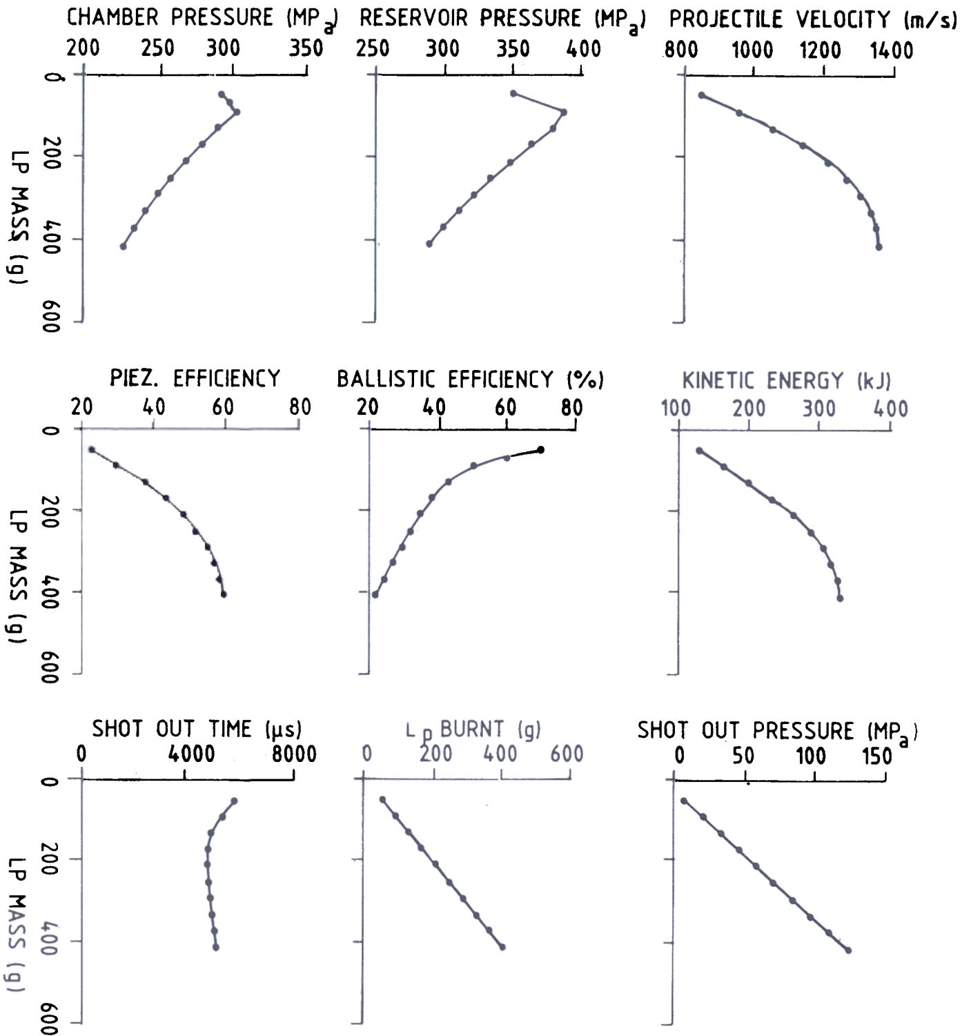
Figure 5. Parametric study for the effect of gun performance with variation of the mass of the liquid propellant.
