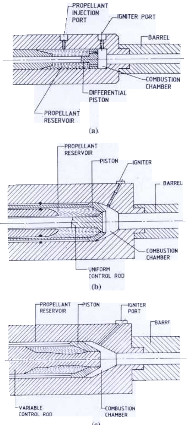
Figure 1 Regenerative liquid propellant guns modelled (a) simple in-line regenerative piston; in-line annular piston with (b) uniform; and (c) variable control rod.
