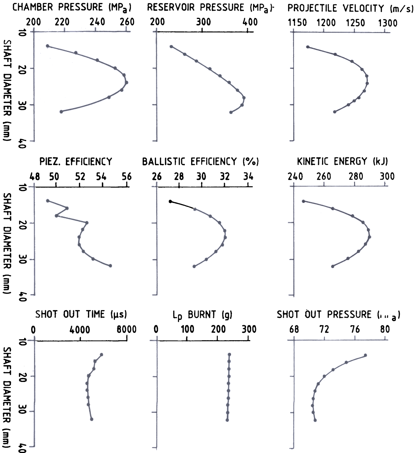
Figure 6. Parametric study for the effect of gun performance with variation in the diameter of piston shaft.
