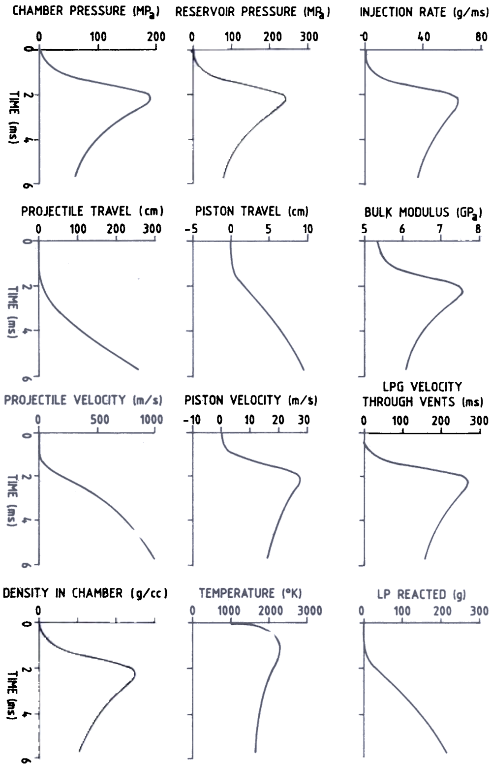
Figure 2. Time evolution of different parameters in the gun (Results obtained using input data of Table 1).
