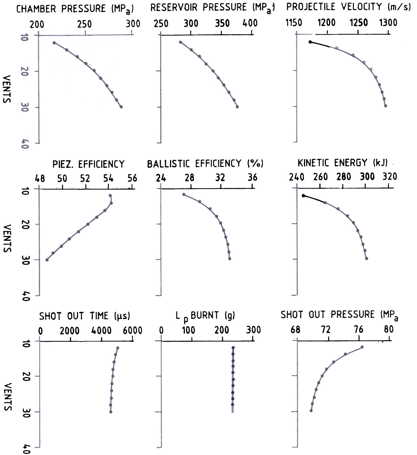
Figure 4. Parametric study for the effect of gun performance with variation in the vent area.
