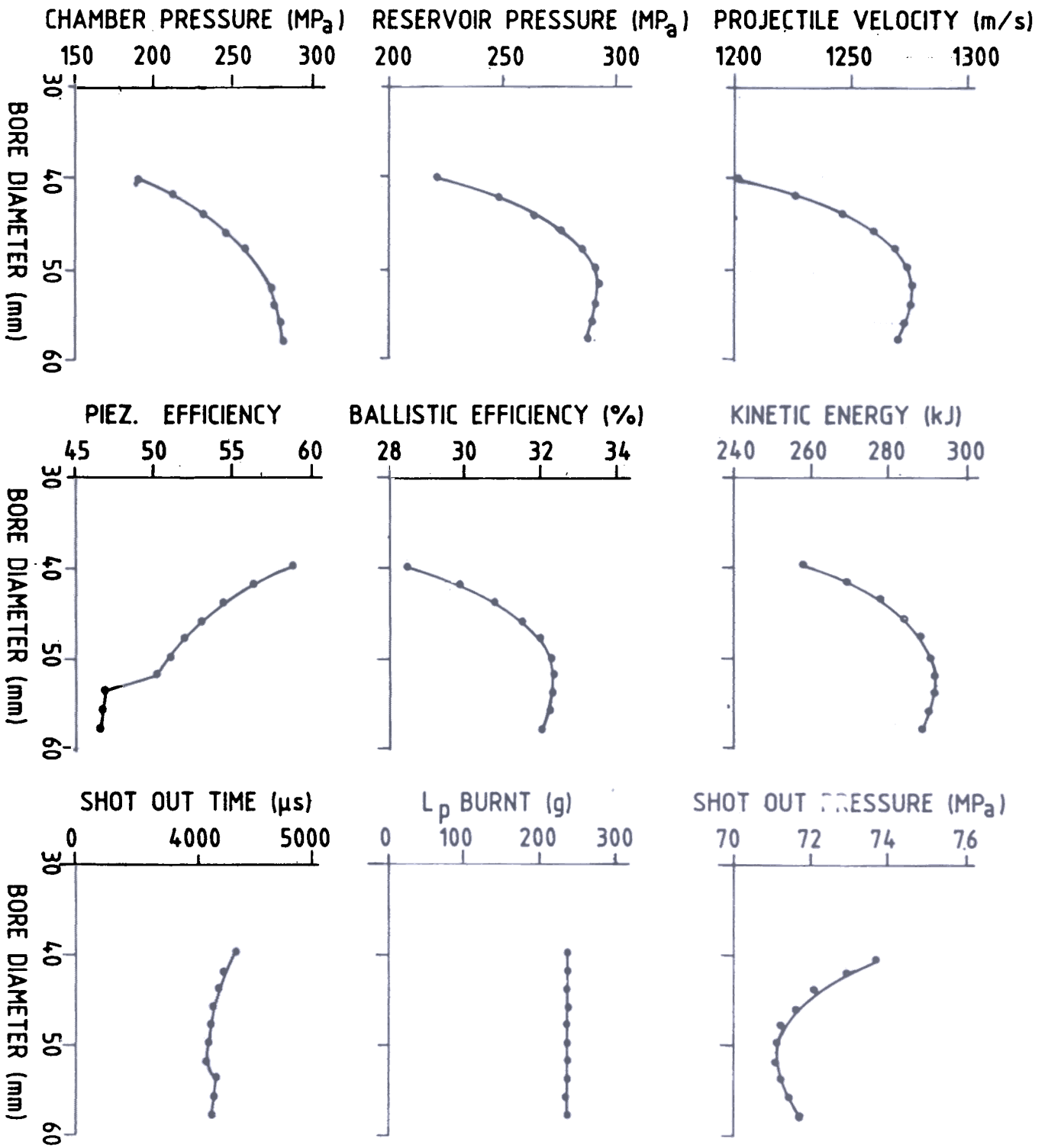
Figure 3. Parametric study for the effect of gun performance with variation in the chamber bore.
