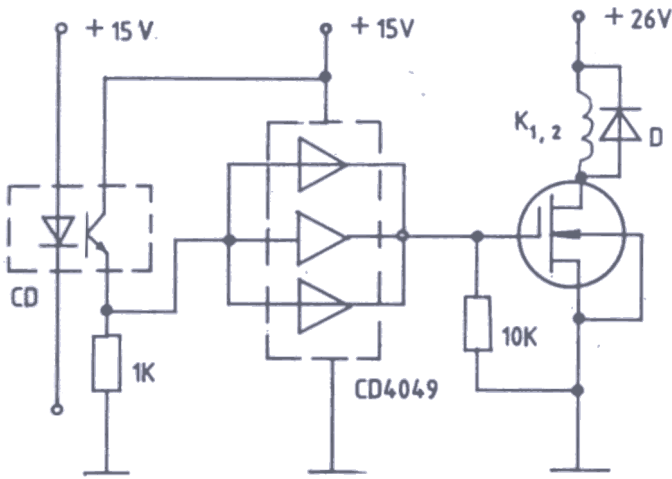
Figure 5 Driving circuit of VMOS transistor
