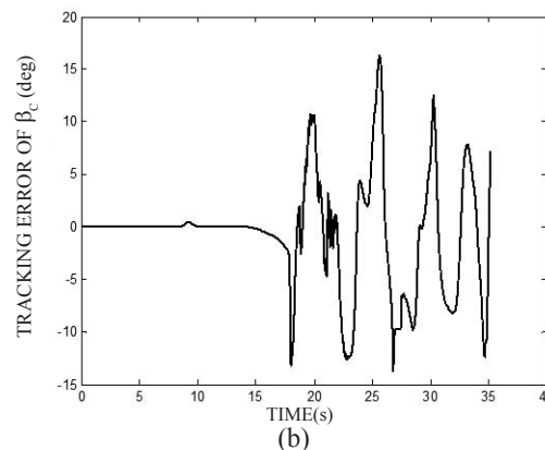
Figure 9. Tracking performance with command of sideslip angle; (a) curves of \beta and \beta_c , (b) tracking error with \beta_c .
