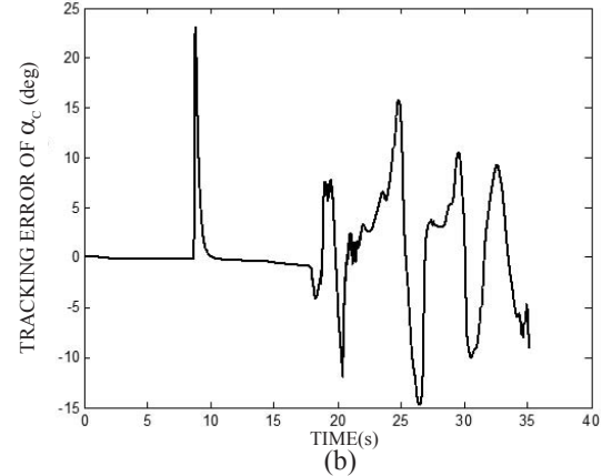
Figure 8. Tracking performance with command angle of attack; (a) curves of \alpha and \alpha_c , (b) tracking error with \alpha_c .
