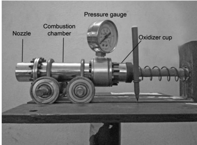
Figure 3. Schematic of hybrid test motor.
