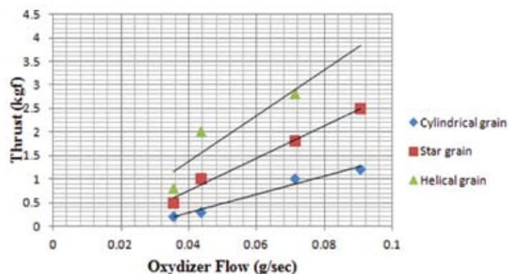
Figure 14. Effect of oxygen flow on thrust for various grain geometries.
