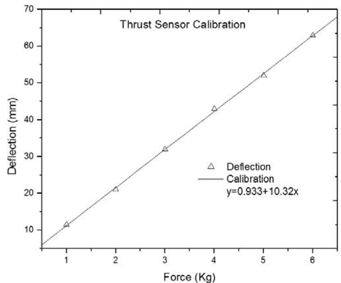
Figure 4. Calibration of the thrust sensors.
