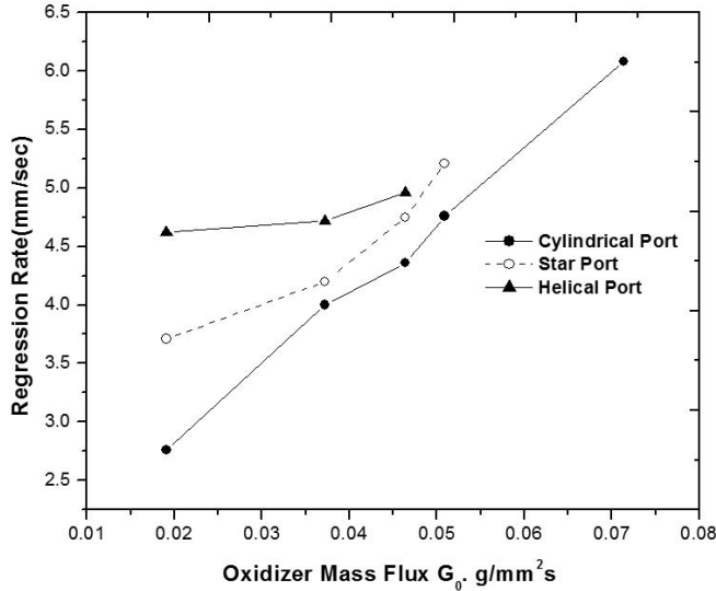
Figure 9. Effect of different grain configuration on regression rate of fuel.
