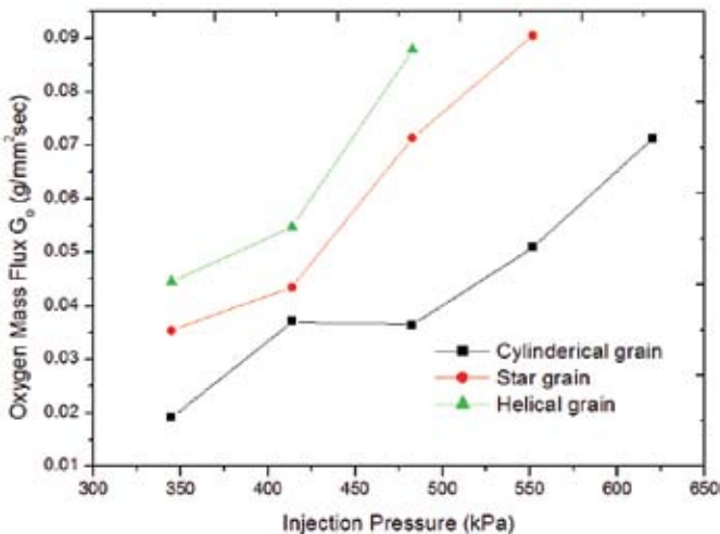
Figure 10. Effect of G_{ox} injection pressure on regression rate.
