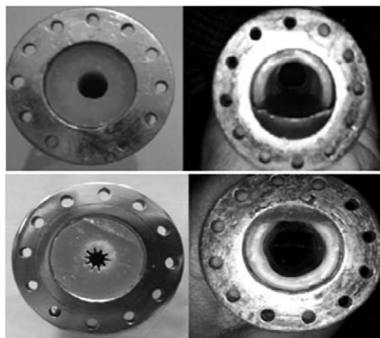
Figure 2. Pre- and post-test result for cylindrical and star paraffin fuel grains.
