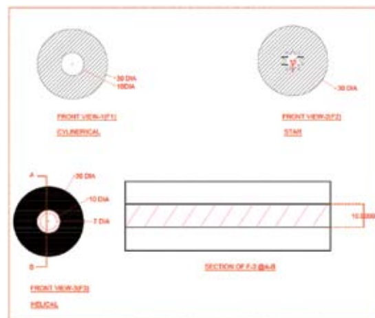
Figure 1. Solid fuel grain configuration.
