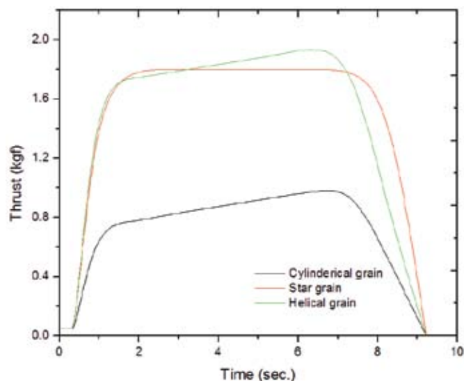
Figure 12. Thrust-time traces for 482.6 kPa.
