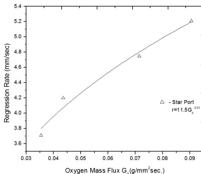
Figure 7. Regression rate variation for star grain with oxidizer mass flux.
