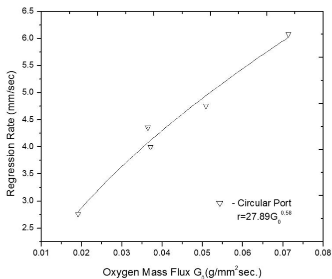
Figure 6. Regression rate variation for cylindrical grain with oxidizer mass flux.
