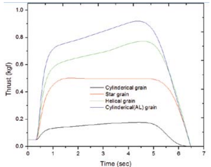
Figure 11. Thrust-time traces for 344.7 kPa.
