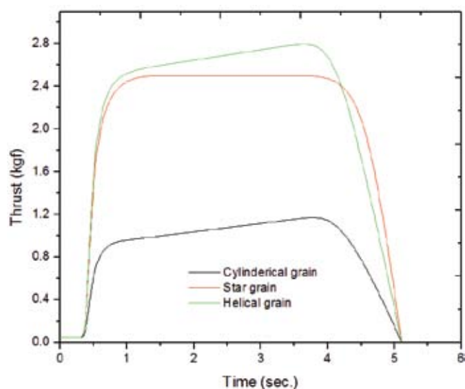
Figure 13. Thrust-time traces for 551.5 kPa.
