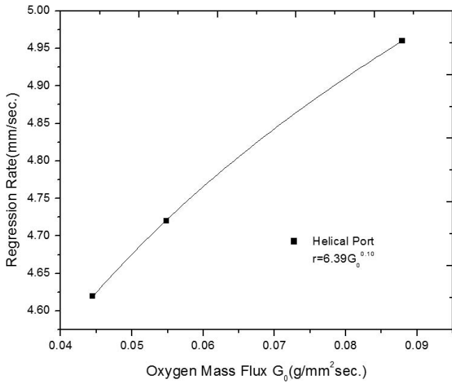
Figure 8. Regression rate variation for helical grain with oxidiser mass flux.
