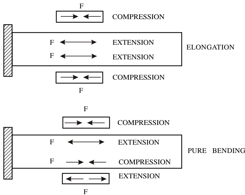
Figure 4. Simple block force model actuators on both surfaces.
