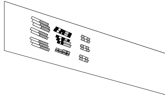
Figure 5. Combination of PZT patches 43 .
