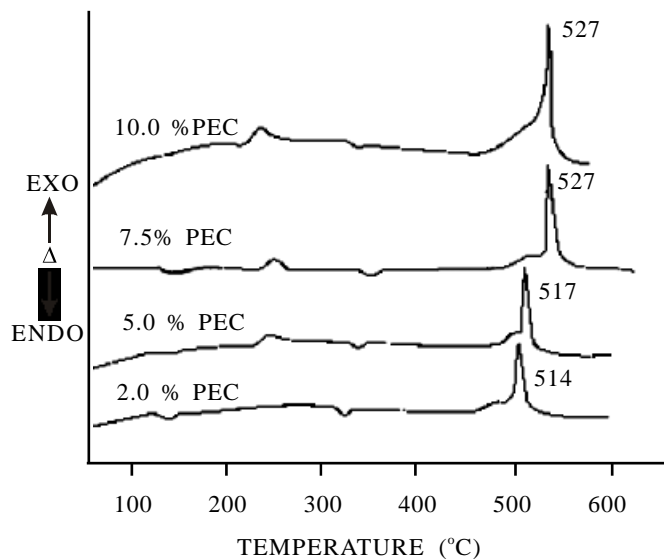
Figure 6. DTA curves of B-KNO_3 system with various percentage of PEC binder atmospheric static air, HR 10 °C/min.
