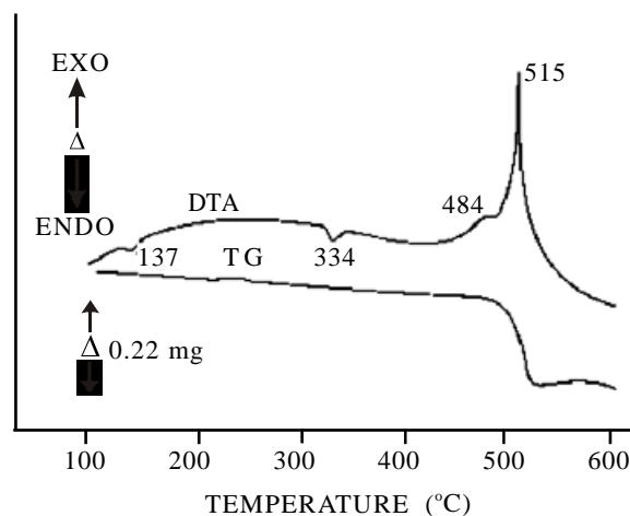
Figure 3. STA curves of B-KNO_3 -NC composition atmospheric static air, HR 10 °C/min.
