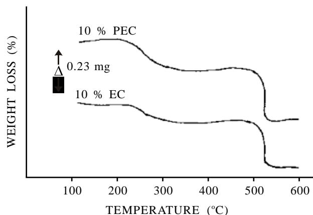
Figure 5. TG curves of B-KNO_3 system with different binders, HR 10 °C/min.
