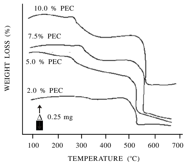
Figure 7. TG curves of B-KNO_3 system with various percentage of PEC atmospheric static air, HR 10 °C/min.
