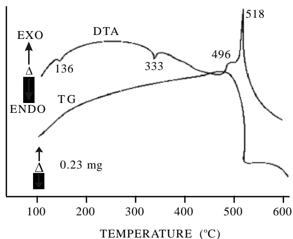
Figure 2. STA curves of B-KNO_3 (1:1) atmospheric static air, HR 10 °C/min.
