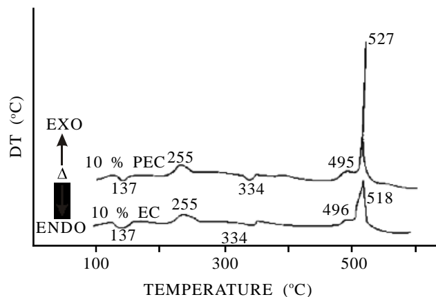
Figure 4. DTA curves of B-KNO_3 system with different binders, HR 10 °C/min.
