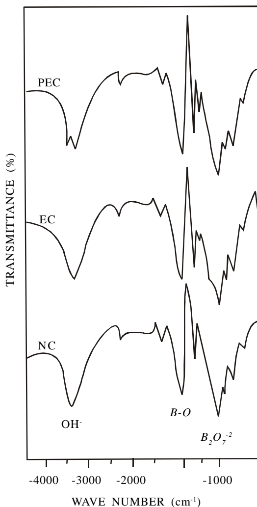
Figure 1. IR spectra of solid combustion products of B-KNO_3 system with different binders.
