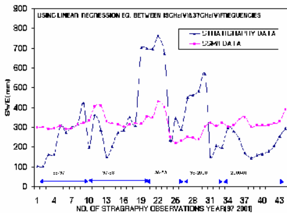
Figure 4. Comparison of SWE between SSM/I and stratigraphy data at Patseo.
