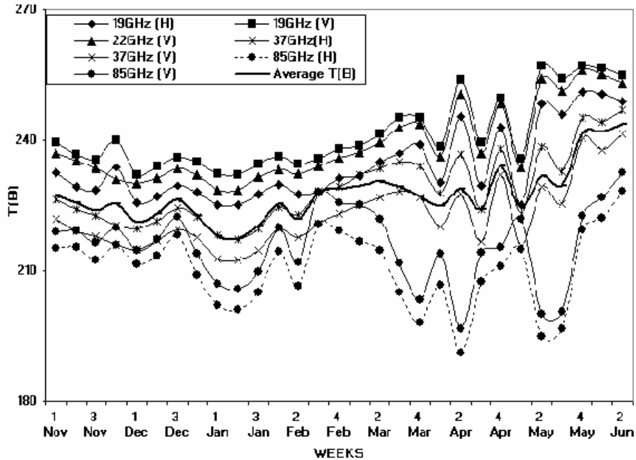
Figure 1. Variation of T_B for 2002-03.
