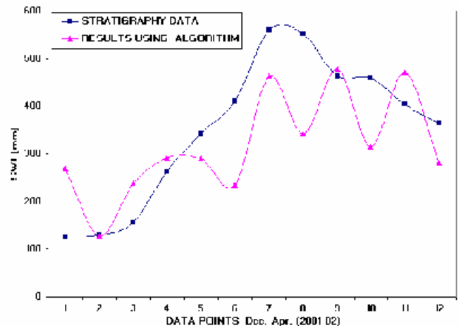
Figure 12. Comparison of SWE based on algorithm and stratigraphy data at Patseo.
