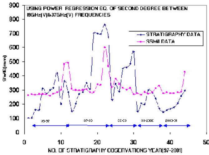
Figure 8. Comparison of SWE between stratigraphy and SSM/I data at Patseo.
