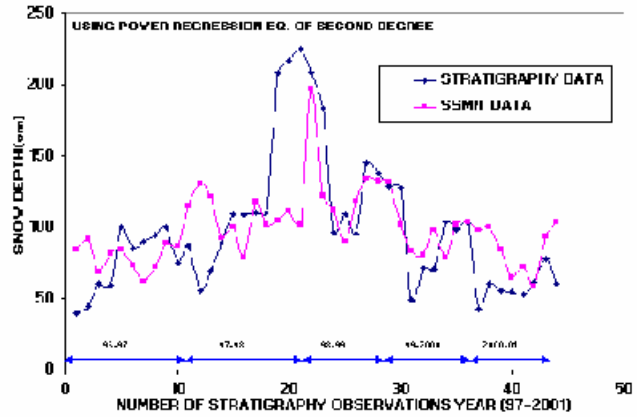
Figure 9. Comparison of snow depth between stratigraphy and SSM/I data at Patseo.
