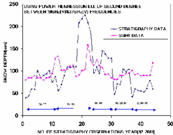
Figure 7. Comparison of snow depth between stratigraphy and SSM/I data at Patseo.
