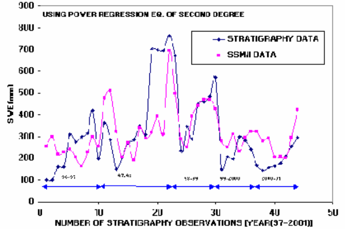
Figure 10. Comparison of SWE between stratigraphy data and SSM/I data at Patseo.
