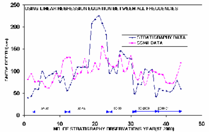
Figure 5. Comparison of snow depth between SSM/I and stratigraphy data at Patseo.
