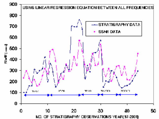
Figure 6. Comparison of SWE between stratigraphy and SSM/I data at Patseo.
