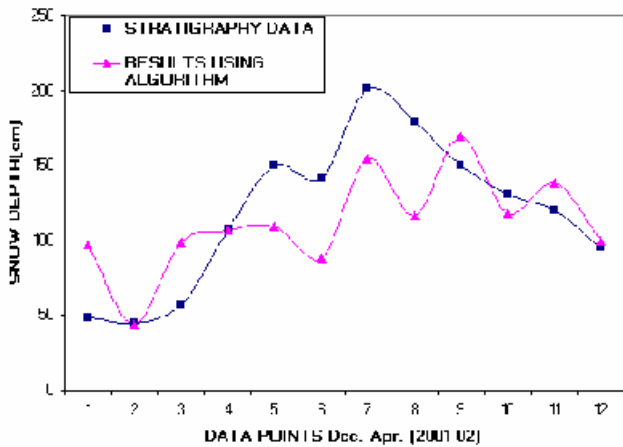
Figure 11. Comparison of snow depth based on algorithm and stratigraphy data.
