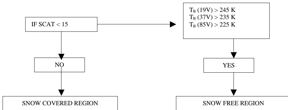
Figure 2. Decision tree for snow identification.
