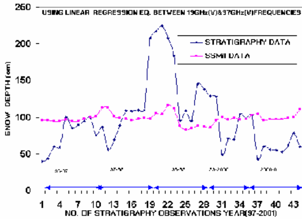
Figure 3. Comparison of snow depth between stratigraphy and SSM/I data at Patseo.
