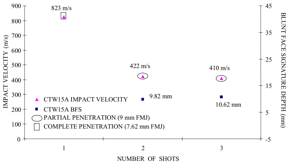
Figure 10. Graphical representation of data points used to determine the ballistic limit for CTW 15A panel using 7.62 mm and 9 mm ammunitions.
