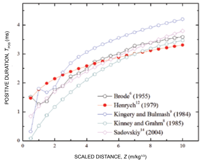
Figure 4. Variation of positive over pressure duration with scaled distance
