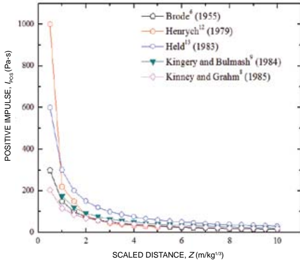
Figure 5. Variation of impulse with scaled distance.
