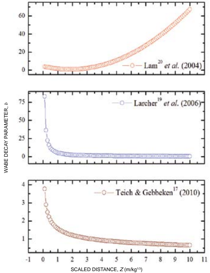
Figure 7. Variation of wave decay parameter with scaled distance.
