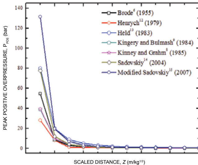
Figure 3. Variation of peak over pressure with scaled distance.
