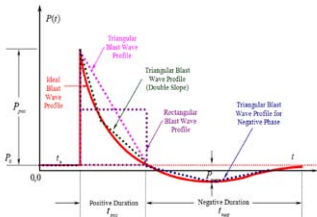
Figure 8. Modified blast wave profile using triangular shape for both positive and negative phase.
