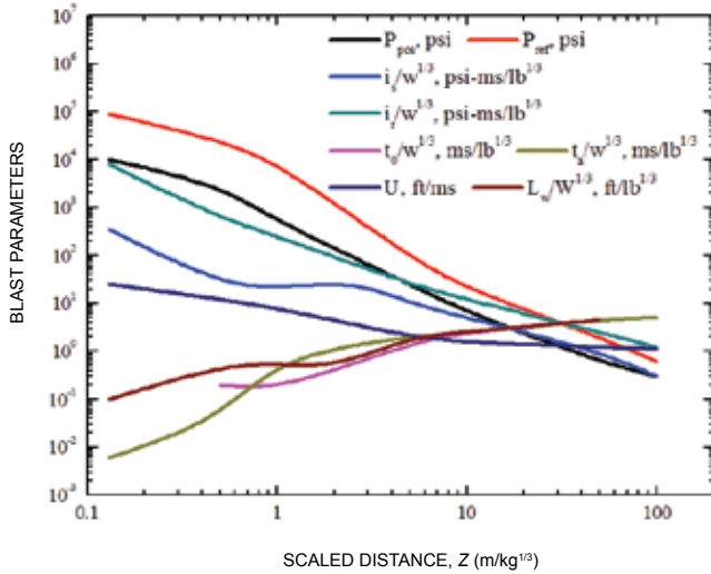
Figure 2. Various blast wave parameters for spherical explosion in air (units in United States customary system).
