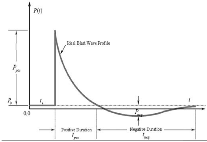
Figure 1. Ideal blast wave resulting from explosion in air.
